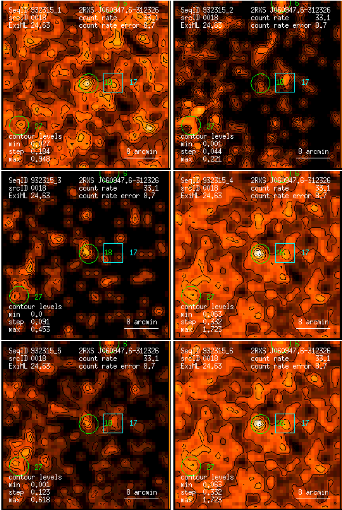
Figure 18: RASS 932315: detection 0018: band rate images, Gaussian filter: (1) PSPC channels 11 – 41, (2) 52 – 90, (3) 91 – 201, (4) 11 – 235, (5) 52 – 201, (6) 11 – 201. Broad band rates in counts/ks. Band rate contour levels in counts/ks/arcmin 2 .
