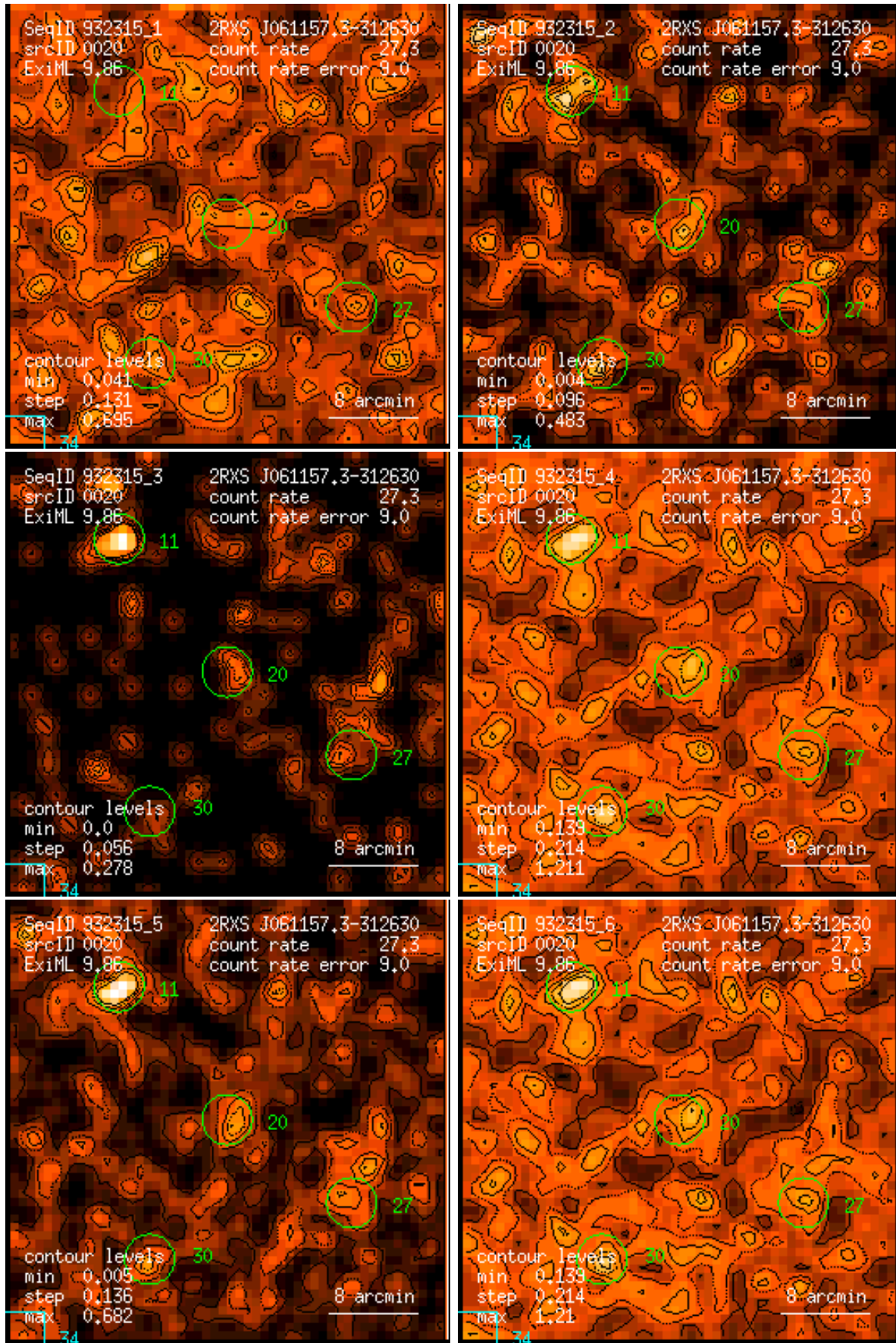
Figure 20: RASS 932315: detection 0020: band rate images, Gaussian filter: (1) PSPC channels 11 – 41, (2) 52 – 90, (3) 91 – 201, (4) 11 – 235, (5) 52 – 201, (6) 11 – 201. Broad band rates in counts/ks. Band rate contour levels in counts/ks/arcmin 2 .
