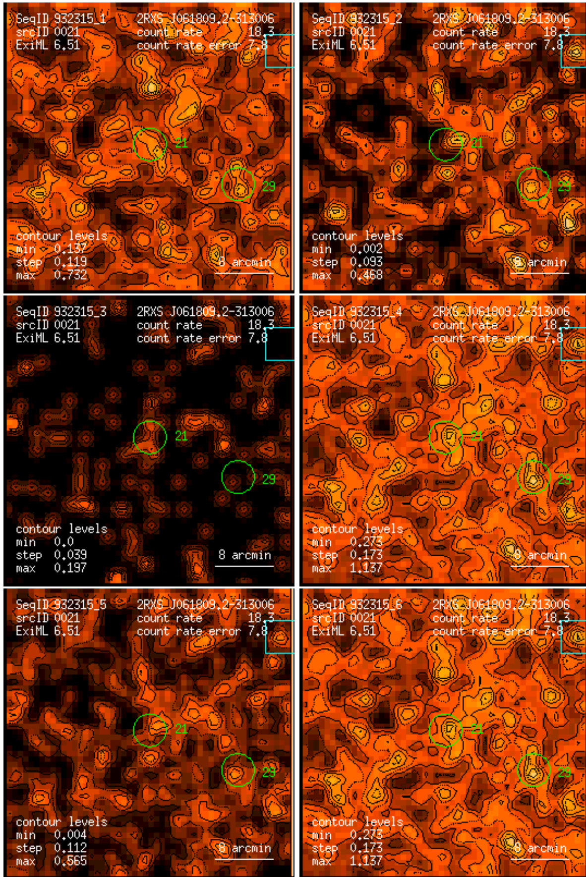
Figure 21: RASS 932315: detection 0021: band rate images, Gaussian filter: (1) PSPC channels 11 – 41, (2) 52 – 90, (3) 91 – 201, (4) 11 – 235, (5) 52 – 201, (6) 11 – 201. Broad band rates in counts/ks. Band rate contour levels in counts/ks/arcmin 2 .
