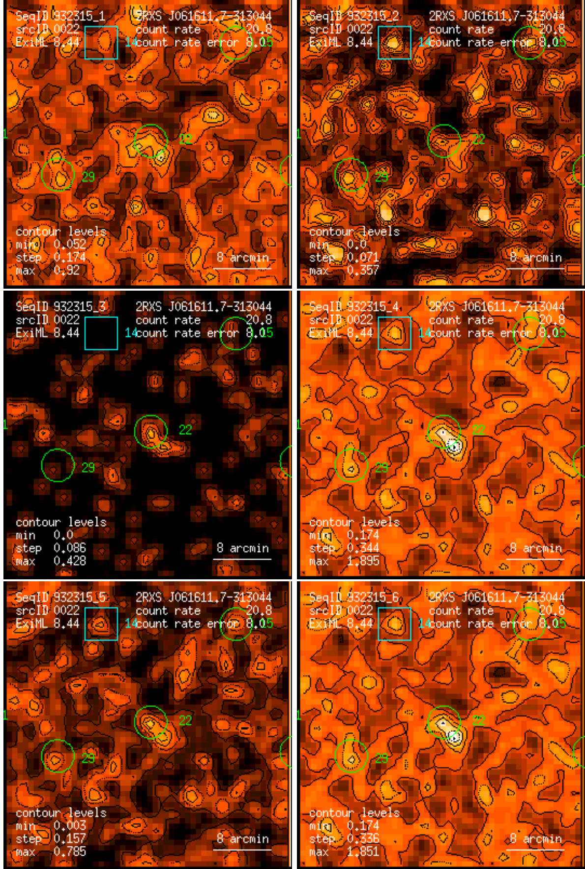
Figure 22: RASS 932315: detection 0022: band rate images, Gaussian filter: (1) PSPC channels 11 – 41, (2) 52 – 90, (3) 91 – 201, (4) 11 – 235, (5) 52 – 201, (6) 11 – 201. Broad band rates in counts/ks. Band rate contour levels in counts/ks/arcmin 2 .
