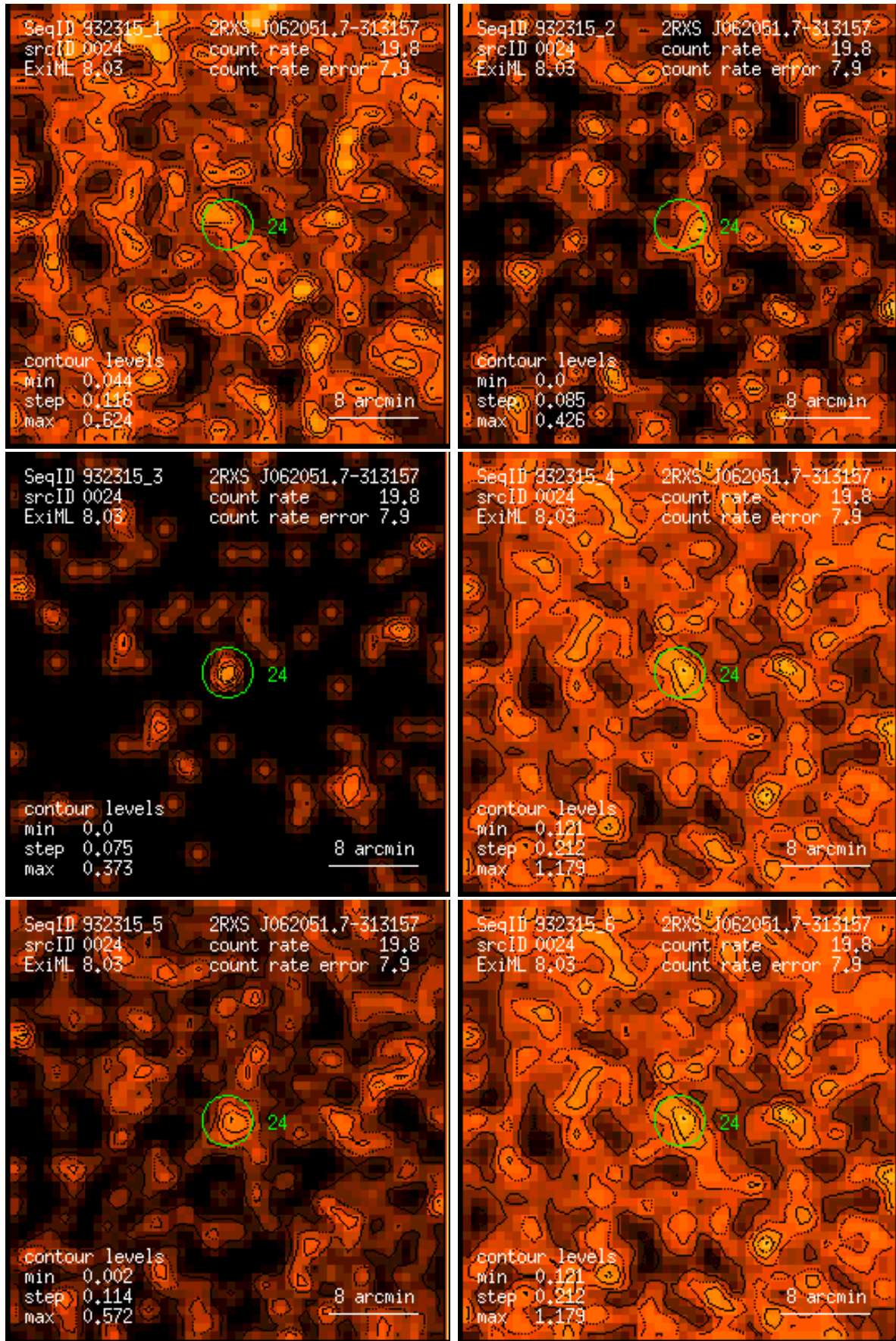
Figure 24: RASS 932315: detection 0024: band rate images, Gaussian filter: (1) PSPC channels 11 – 41, (2) 52 – 90, (3) 91 – 201, (4) 11 – 235, (5) 52 – 201, (6) 11 – 201. Broad band rates in counts/ks. Band rate contour levels in counts/ks/arcmin 2 .
