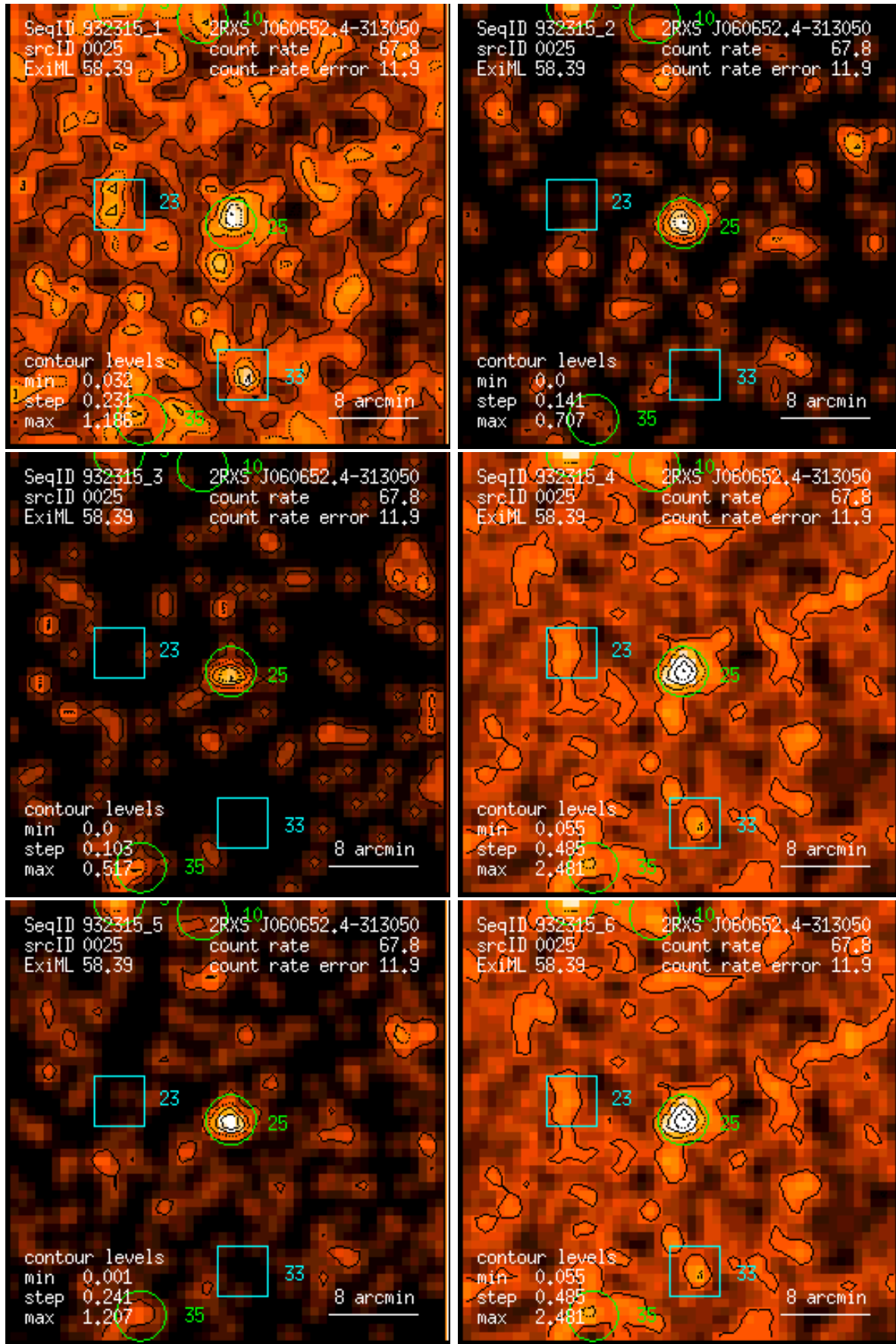
Figure 25: RASS 932315: detection 0025: band rate images, Gaussian filter: (1) PSPC channels 11 – 41, (2) 52 – 90, (3) 91 – 201, (4) 11 – 235, (5) 52 – 201, (6) 11 – 201. Broad band rates in counts/ks. Band rate contour levels in counts/ks/arcmin 2 .
