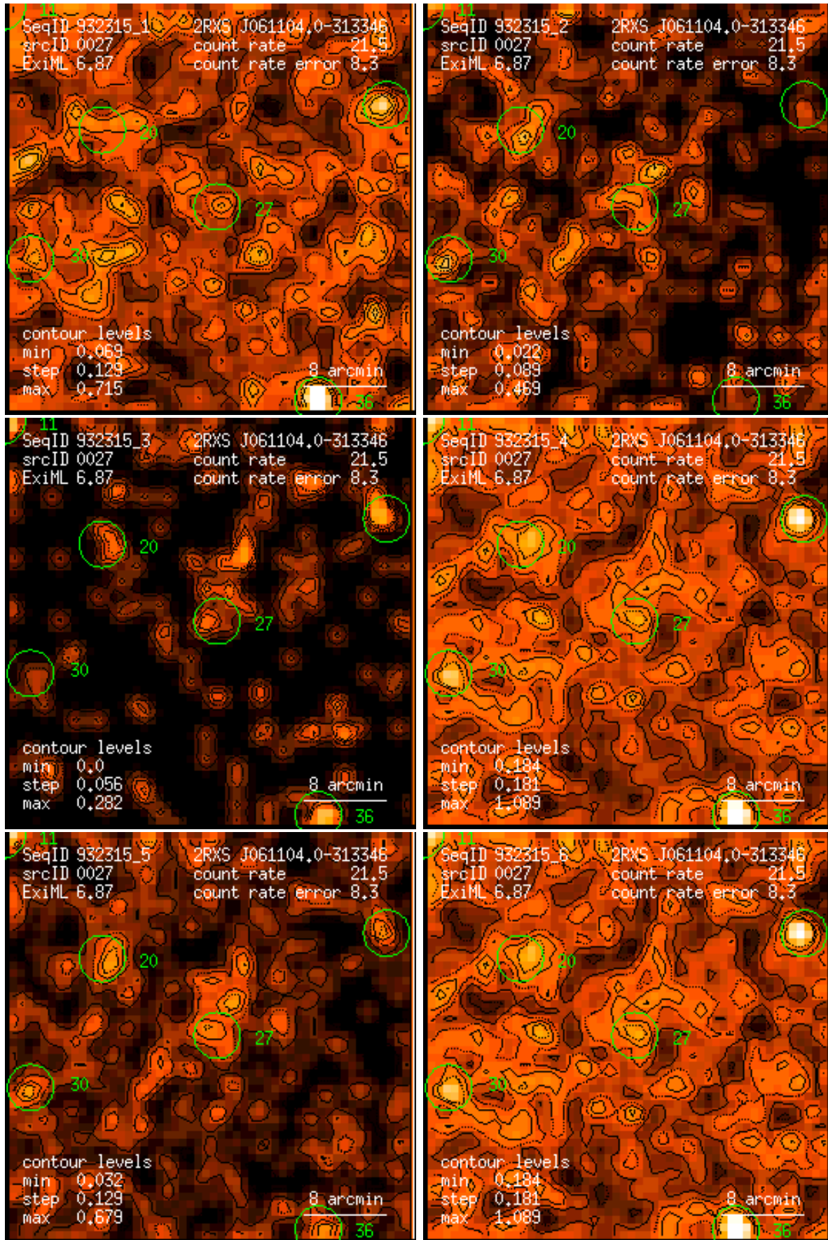
Figure 27: RASS 932315: detection 0027: band rate images, Gaussian filter: (1) PSPC channels 11 – 41, (2) 52 – 90, (3) 91 – 201, (4) 11 – 235, (5) 52 – 201, (6) 11 – 201. Broad band rates in counts/ks. Band rate contour levels in counts/ks/arcmin 2 .
