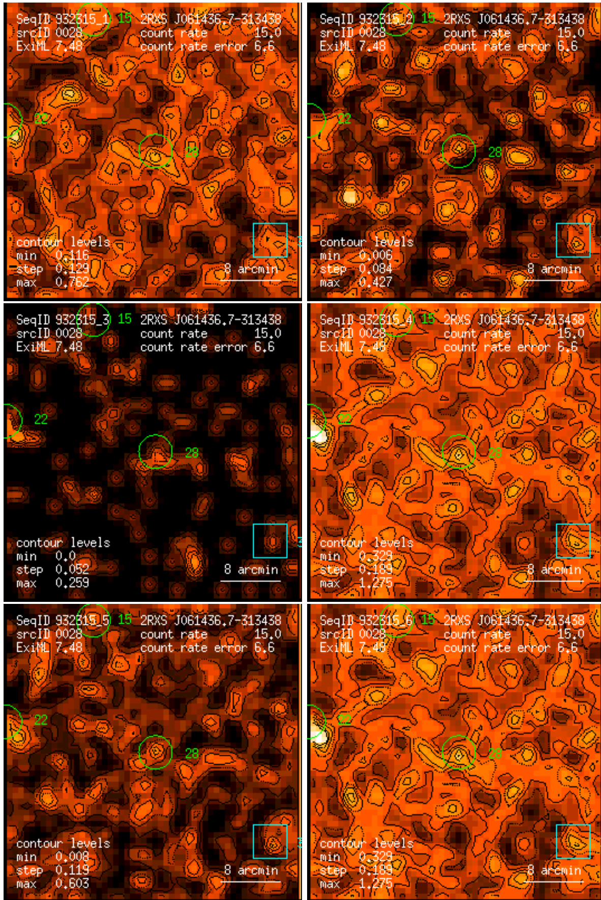
Figure 28: RASS 932315: detection 0028: band rate images, Gaussian filter: (1) PSPC channels 11 – 41, (2) 52 – 90, (3) 91 – 201, (4) 11 – 235, (5) 52 – 201, (6) 11 – 201. Broad band rates in counts/ks. Band rate contour levels in counts/ks/arcmin 2 .
