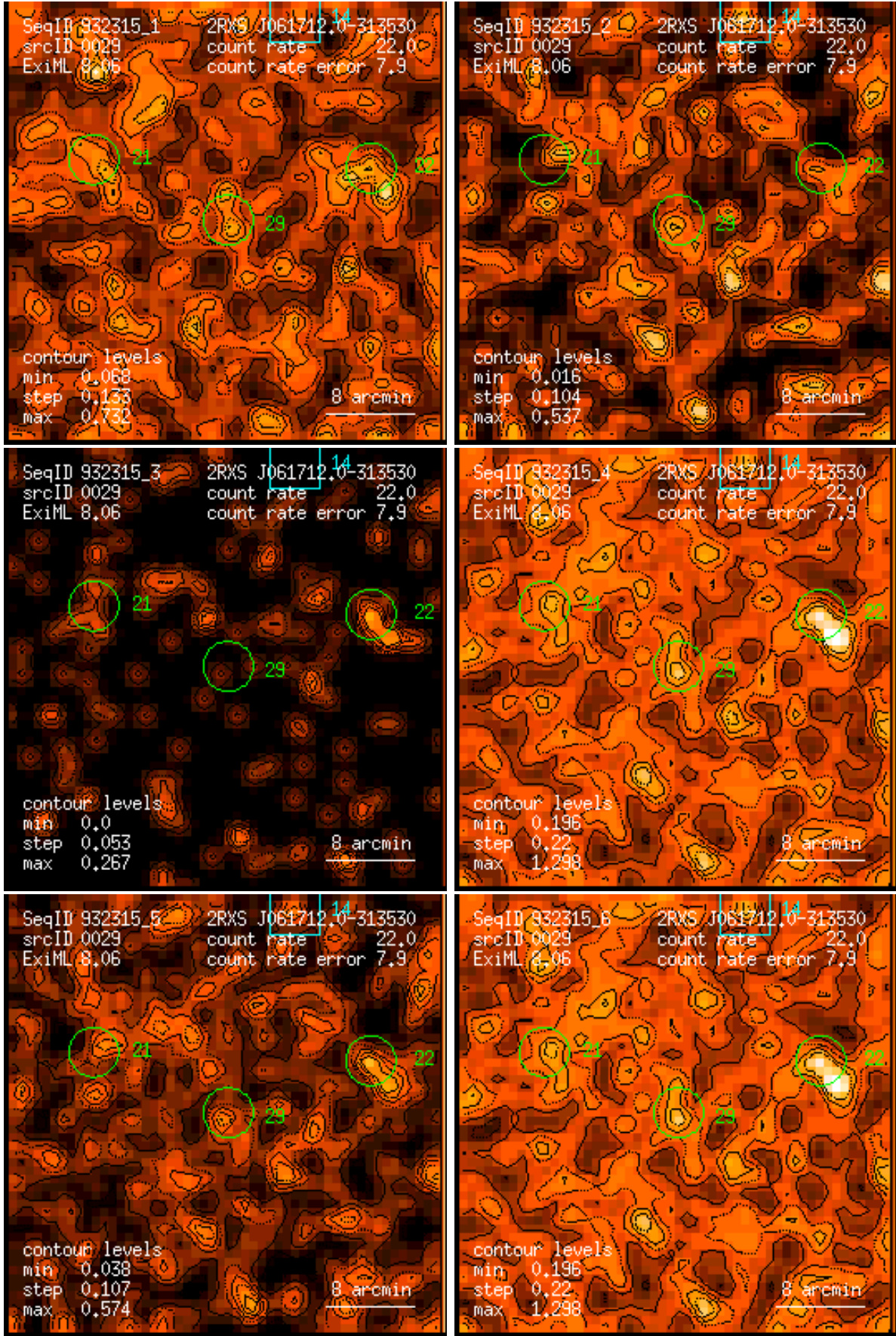
Figure 29: RASS 932315: detection 0029: band rate images, Gaussian filter: (1) PSPC channels 11 – 41, (2) 52 – 90, (3) 91 – 201, (4) 11 – 235, (5) 52 – 201, (6) 11 – 201. Broad band rates in counts/ks. Band rate contour levels in counts/ks/arcmin 2 .
