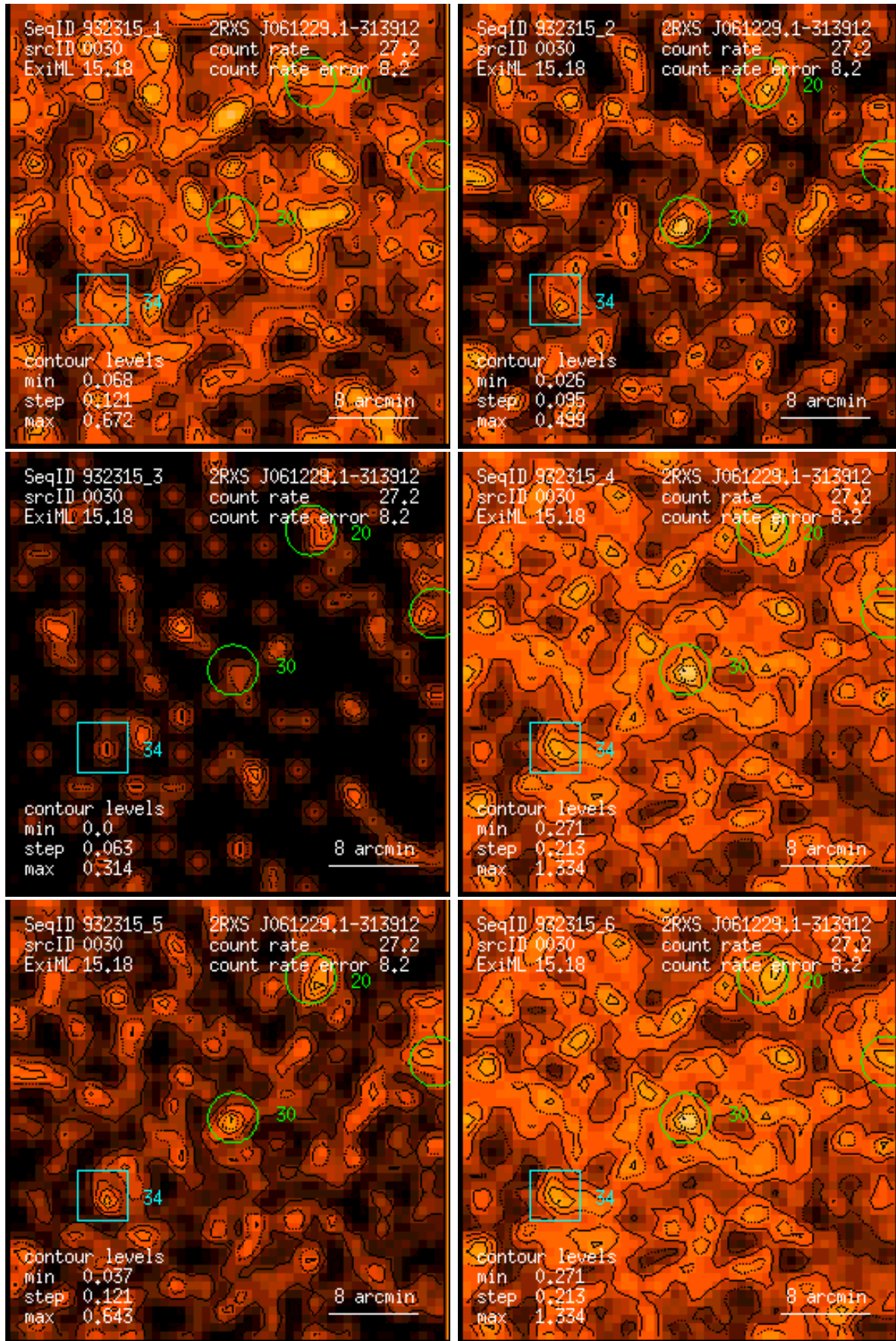
Figure 30: RASS 932315: detection 0030: band rate images, Gaussian filter: (1) PSPC channels 11 – 41, (2) 52 – 90, (3) 91 – 201, (4) 11 – 235, (5) 52 – 201, (6) 11 – 201. Broad band rates in counts/ks. Band rate contour levels in counts/ks/arcmin 2 .
