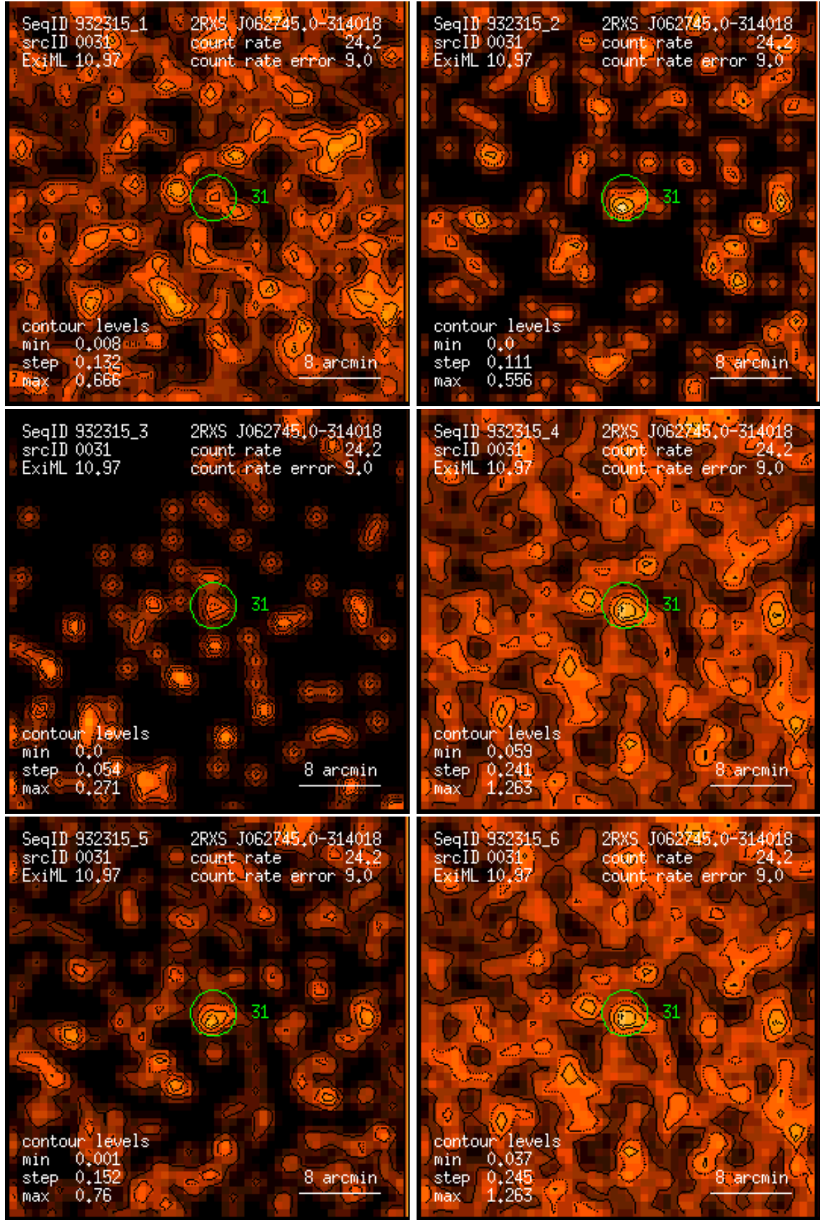
Figure 31: RASS 932315: detection 0031: band rate images, Gaussian filter: (1) PSPC channels 11 – 41, (2) 52 – 90, (3) 91 – 201, (4) 11 – 235, (5) 52 – 201, (6) 11 – 201. Broad band rates in counts/ks. Band rate contour levels in counts/ks/arcmin 2 .
