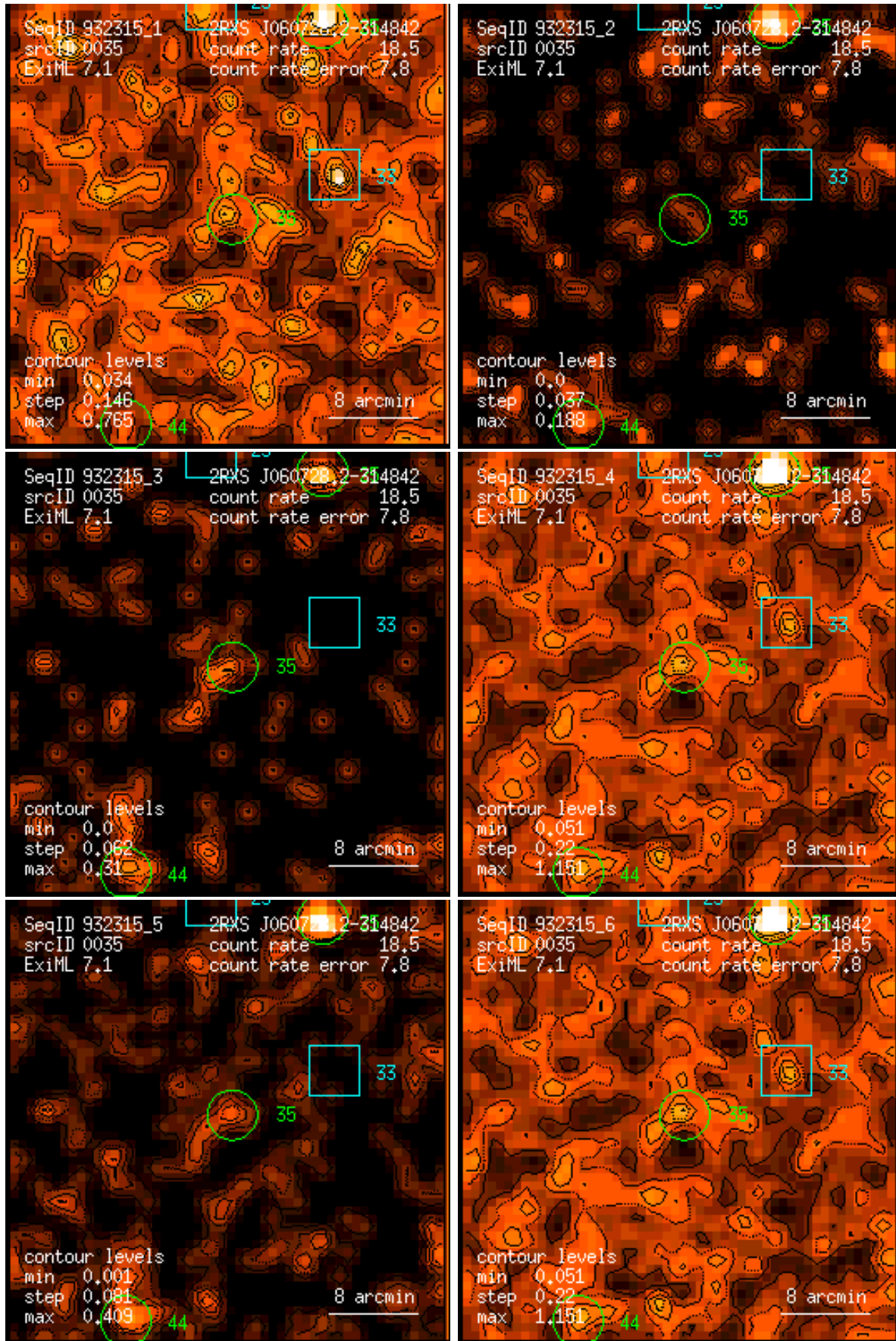
Figure 35: RASS 932315: detection 0035: band rate images, Gaussian filter: (1) PSPC channels 11 – 41, (2) 52 – 90, (3) 91 – 201, (4) 11 – 235, (5) 52 – 201, (6) 11 – 201. Broad band rates in counts/ks. Band rate contour levels in counts/ks/arcmin 2 .
