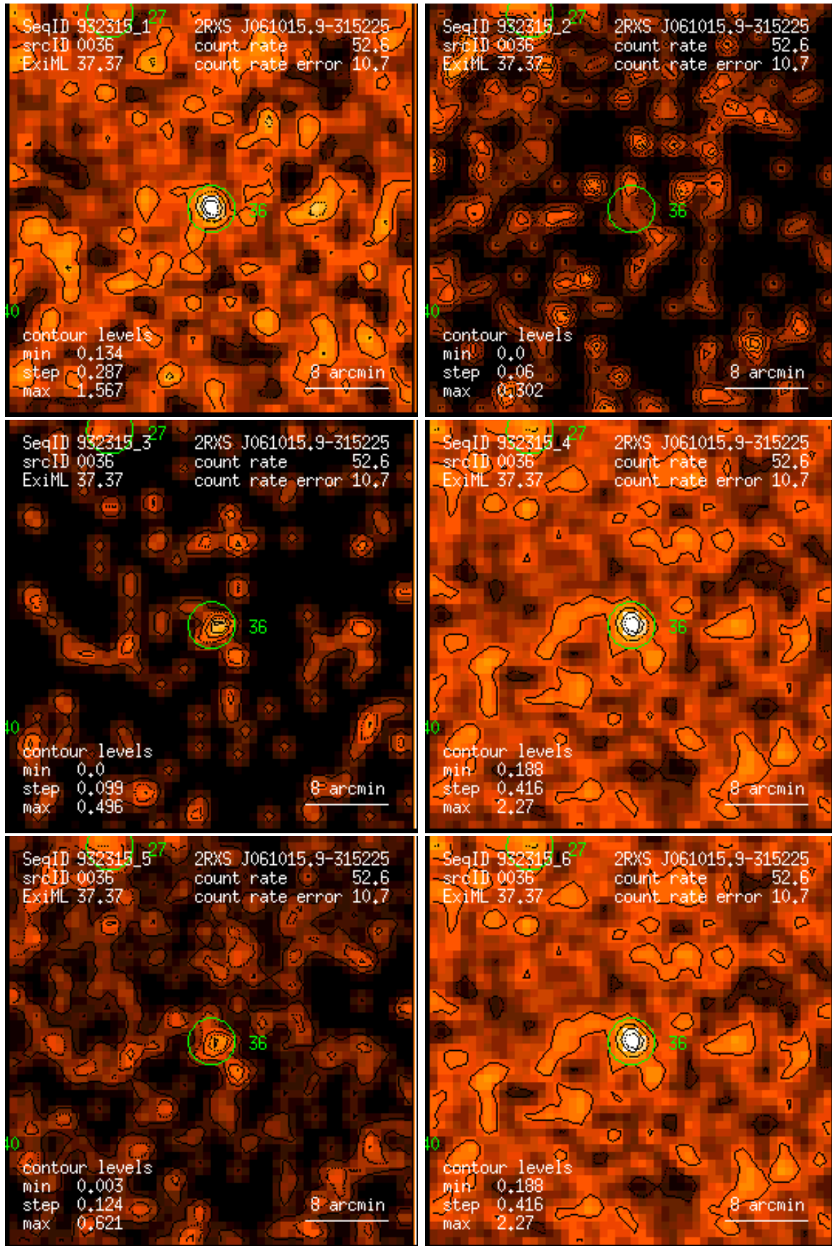
Figure 36: RASS 932315: detection 0036: band rate images, Gaussian filter: (1) PSPC channels 11 – 41, (2) 52 – 90, (3) 91 – 201, (4) 11 – 235, (5) 52 – 201, (6) 11 – 201. Broad band rates in counts/ks. Band rate contour levels in counts/ks/arcmin 2 .
