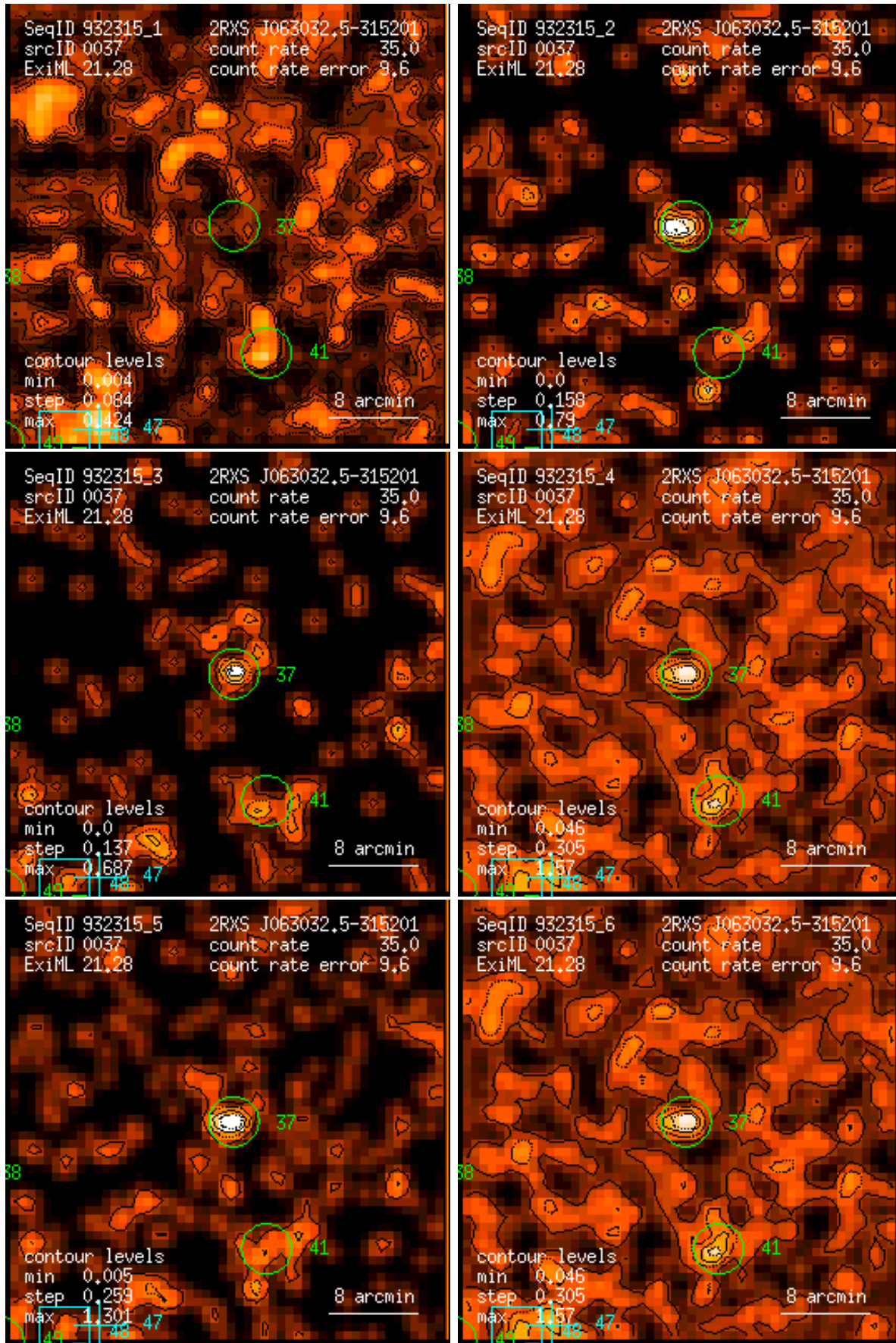
Figure 37: RASS 932315: detection 0037: band rate images, Gaussian filter: (1) PSPC channels 11 – 41, (2) 52 – 90, (3) 91 – 201, (4) 11 – 235, (5) 52 – 201, (6) 11 – 201. Broad band rates in counts/ks. Band rate contour levels in counts/ks/arcmin 2 .
