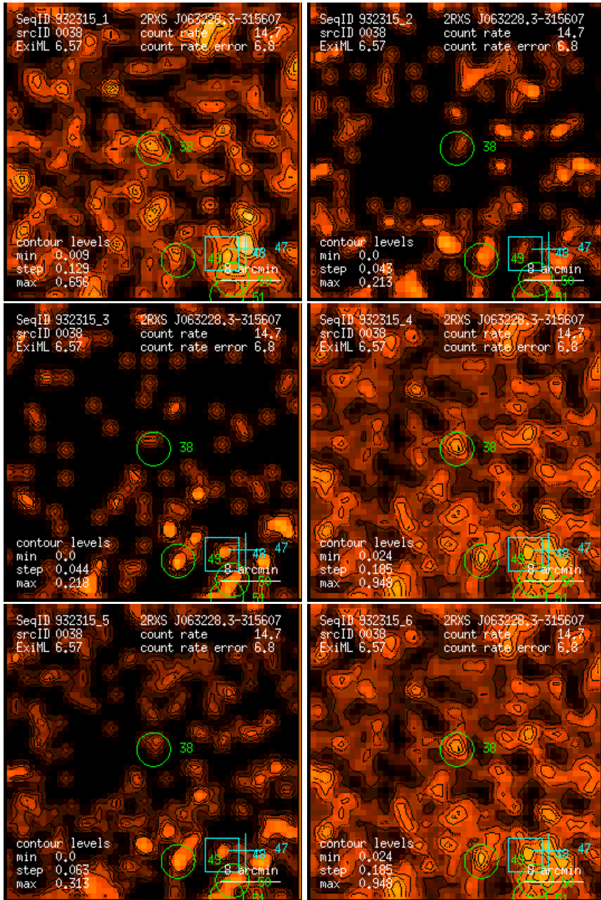
Figure 38: RASS 932315: detection 0038: band rate images, Gaussian filter: (1) PSPC channels 11 – 41, (2) 52 – 90, (3) 91 – 201, (4) 11 – 235, (5) 52 – 201, (6) 11 – 201. Broad band rates in counts/ks. Band rate contour levels in counts/ks/arcmin 2 .
