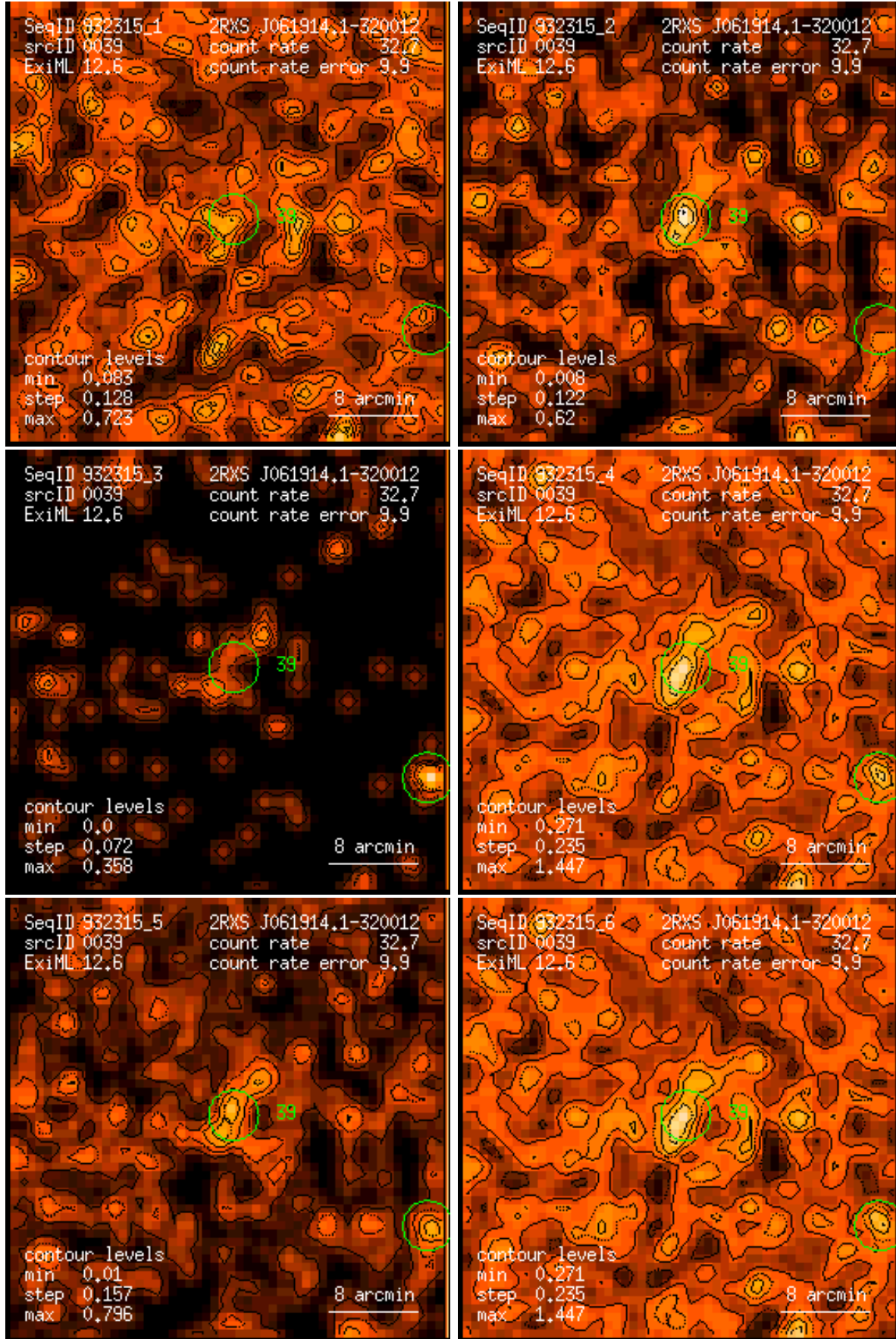
Figure 39: RASS 932315: detection 0039: band rate images, Gaussian filter: (1) PSPC channels 11 – 41, (2) 52 – 90, (3) 91 – 201, (4) 11 – 235, (5) 52 – 201, (6) 11 – 201. Broad band rates in counts/ks. Band rate contour levels in counts/ks/arcmin 2 .
