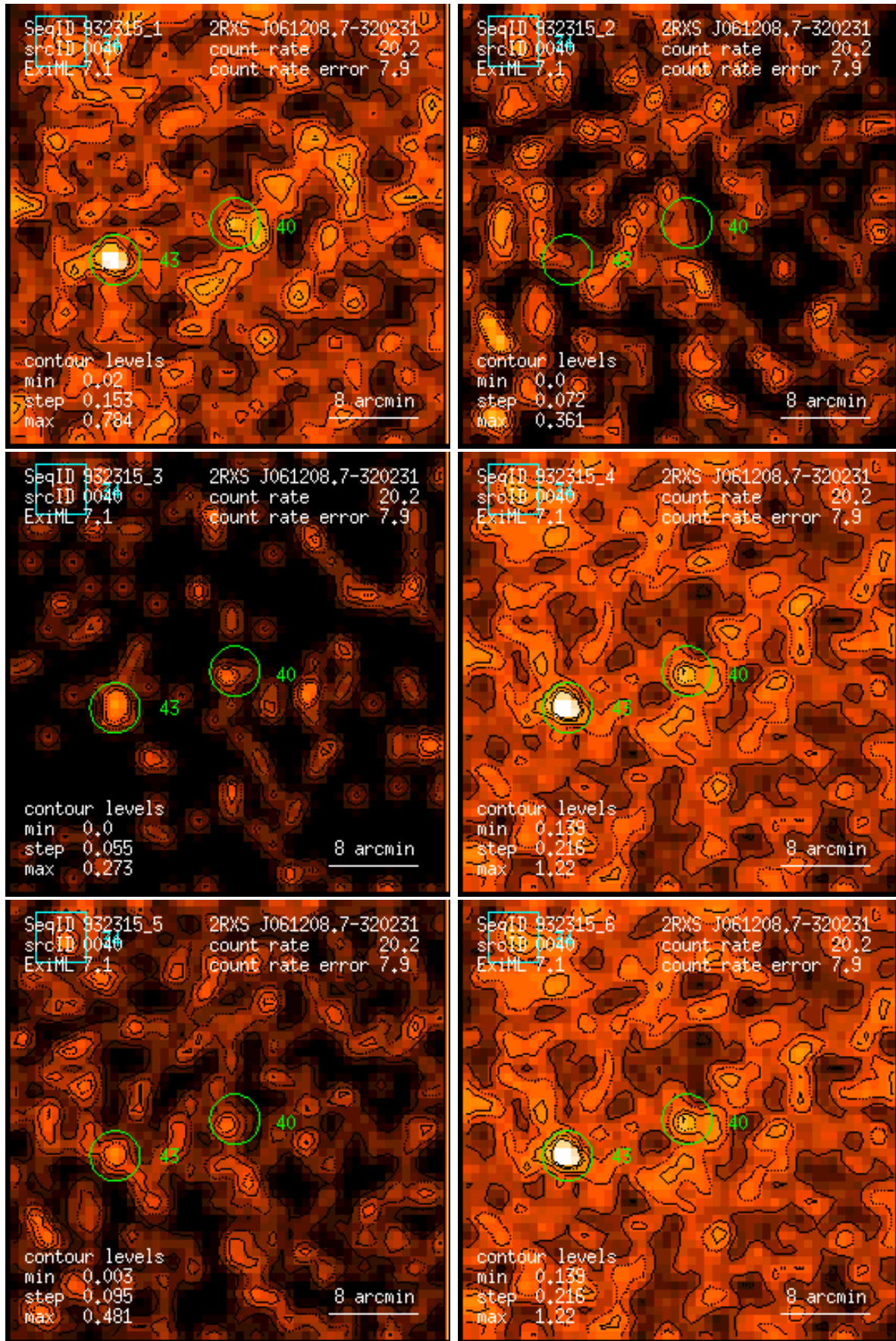
Figure 40: RASS 932315: detection 0040: band rate images, Gaussian filter: (1) PSPC channels 11 – 41, (2) 52 – 90, (3) 91 – 201, (4) 11 – 235, (5) 52 – 201, (6) 11 – 201. Broad band rates in counts/ks. Band rate contour levels in counts/ks/arcmin 2 .
