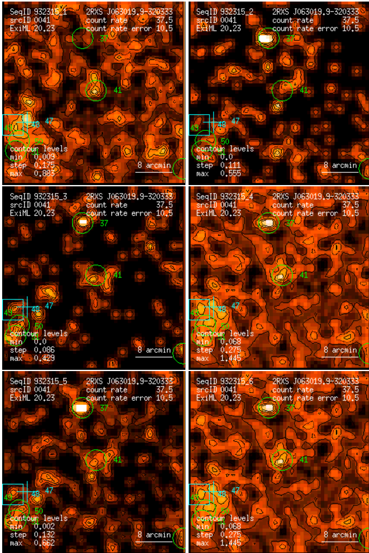
Figure 41: RASS 932315: detection 0041: band rate images, Gaussian filter: (1) PSPC channels 11 – 41, (2) 52 – 90, (3) 91 – 201, (4) 11 – 235, (5) 52 – 201, (6) 11 – 201. Broad band rates in counts/ks. Band rate contour levels in counts/ks/arcmin 2 .
