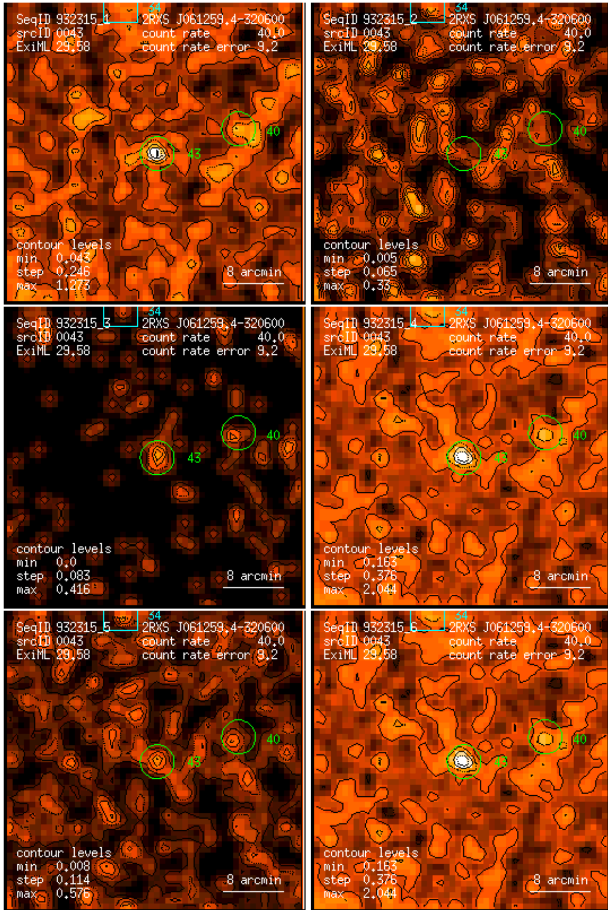
Figure 43: RASS 932315: detection 0043: band rate images, Gaussian filter: (1) PSPC channels 11 – 41, (2) 52 – 90, (3) 91 – 201, (4) 11 – 235, (5) 52 – 201, (6) 11 – 201. Broad band rates in counts/ks. Band rate contour levels in counts/ks/arcmin 2 .
