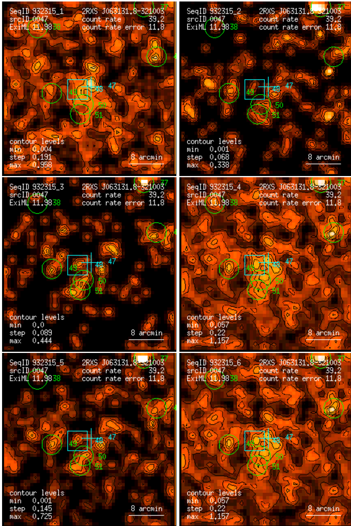
Figure 47: RASS 932315: detection 0047: band rate images, Gaussian filter: (1) PSPC channels 11 – 41, (2) 52 – 90, (3) 91 – 201, (4) 11 – 235, (5) 52 – 201, (6) 11 – 201. Broad band rates in counts/ks. Band rate contour levels in counts/ks/arcmin 2 .
