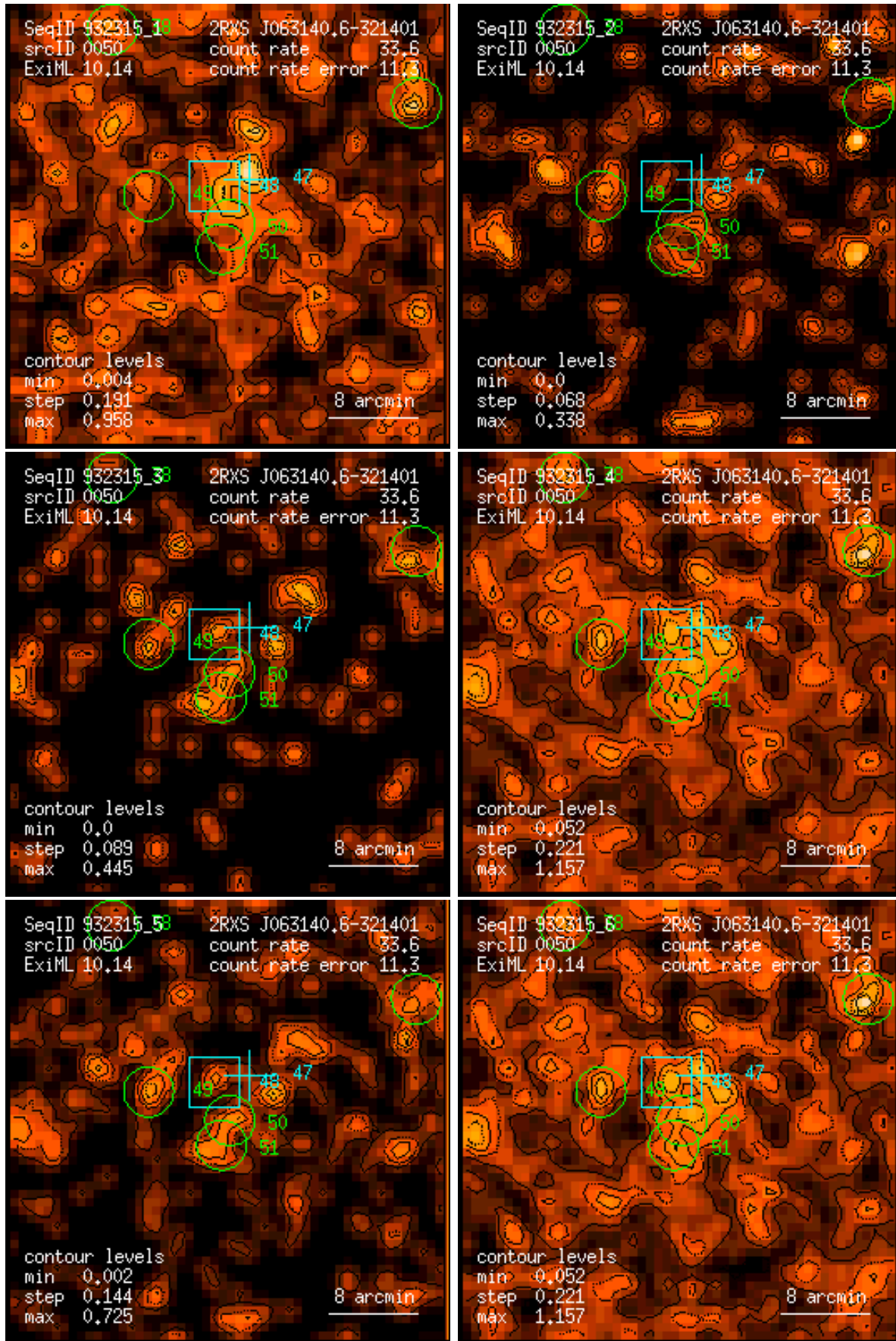
Figure 50: RASS 932315: detection 0050: band rate images, Gaussian filter: (1) PSPC channels 11 – 41, (2) 52 – 90, (3) 91 – 201, (4) 11 – 235, (5) 52 – 201, (6) 11 – 201. Broad band rates in counts/ks. Band rate contour levels in counts/ks/arcmin 2 .
