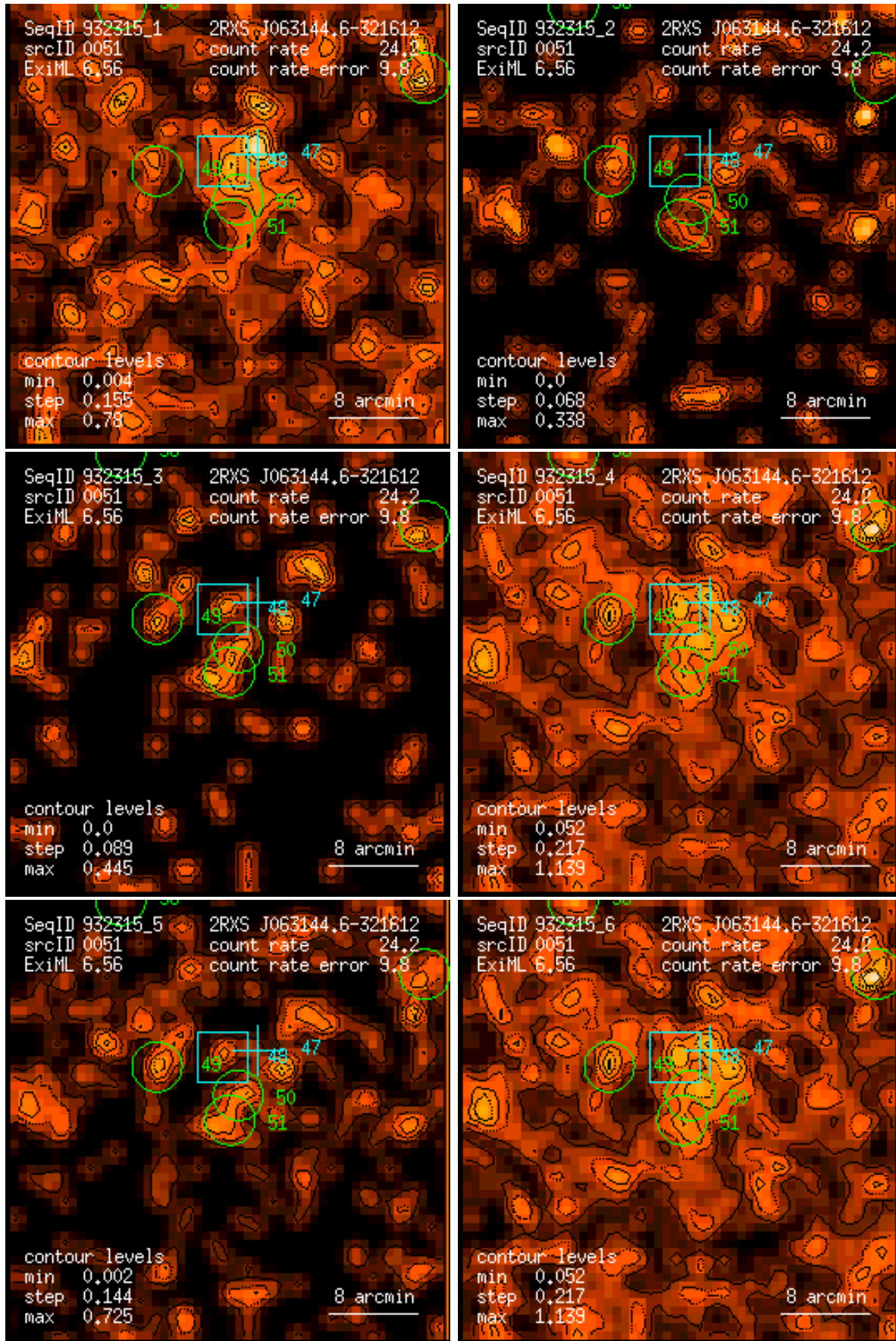
Figure 51: RASS 932315: detection 0051: band rate images, Gaussian filter: (1) PSPC channels 11 – 41, (2) 52 – 90, (3) 91 – 201, (4) 11 – 235, (5) 52 – 201, (6) 11 – 201. Broad band rates in counts/ks. Band rate contour levels in counts/ks/arcmin 2 .
