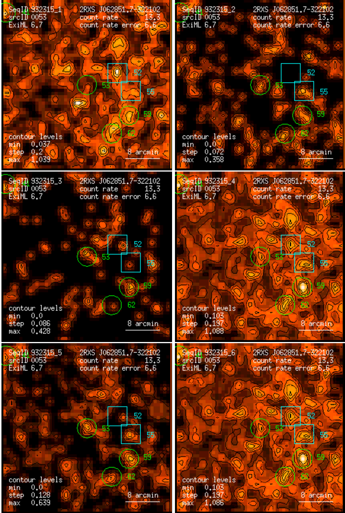
Figure 53: RASS 932315: detection 0053: band rate images, Gaussian filter: (1) PSPC channels 11 – 41, (2) 52 – 90, (3) 91 – 201, (4) 11 – 235, (5) 52 – 201, (6) 11 – 201. Broad band rates in counts/ks. Band rate contour levels in counts/ks/arcmin 2 .
