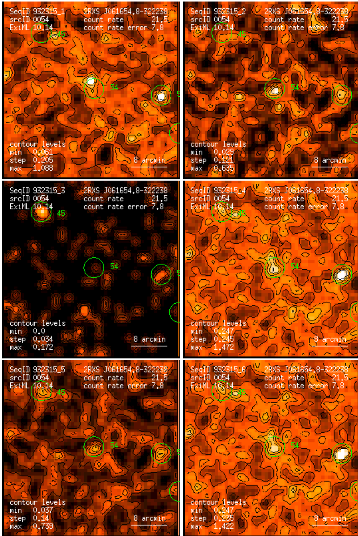
Figure 54: RASS 932315: detection 0054: band rate images, Gaussian filter: (1) PSPC channels 11 – 41, (2) 52 – 90, (3) 91 – 201, (4) 11 – 235, (5) 52 – 201, (6) 11 – 201. Broad band rates in counts/ks. Band rate contour levels in counts/ks/arcmin 2 .
