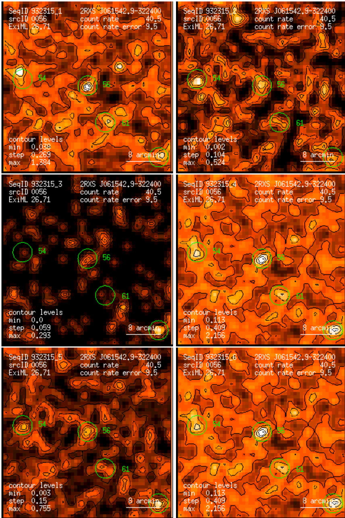
Figure 56: RASS 932315: detection 0056: band rate images, Gaussian filter: (1) PSPC channels 11 – 41, (2) 52 – 90, (3) 91 – 201, (4) 11 – 235, (5) 52 – 201, (6) 11 – 201. Broad band rates in counts/ks. Band rate contour levels in counts/ks/arcmin 2 .
