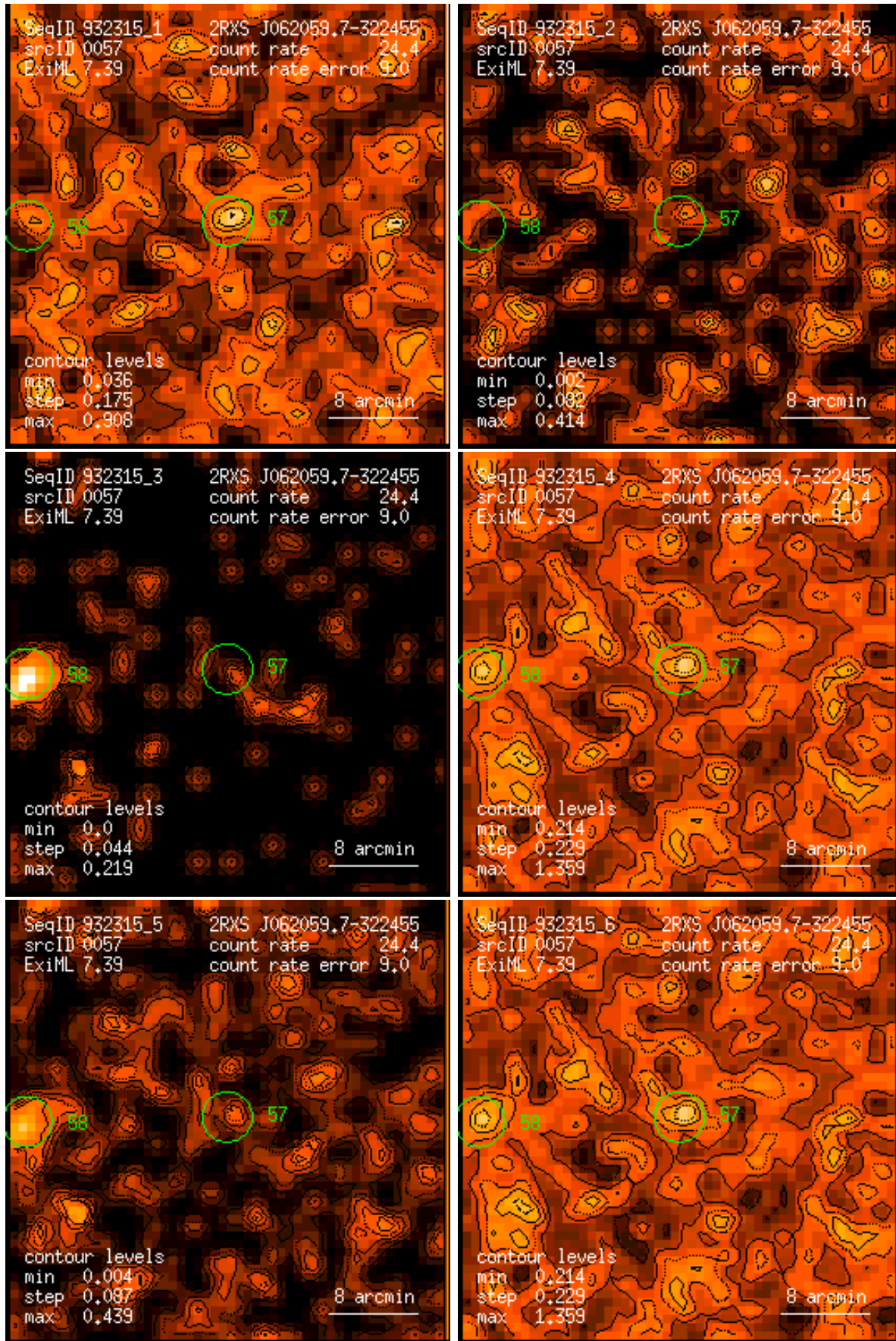
Figure 57: RASS 932315: detection 0057: band rate images, Gaussian filter: (1) PSPC channels 11 – 41, (2) 52 – 90, (3) 91 – 201, (4) 11 – 235, (5) 52 – 201, (6) 11 – 201. Broad band rates in counts/ks. Band rate contour levels in counts/ks/arcmin 2 .
