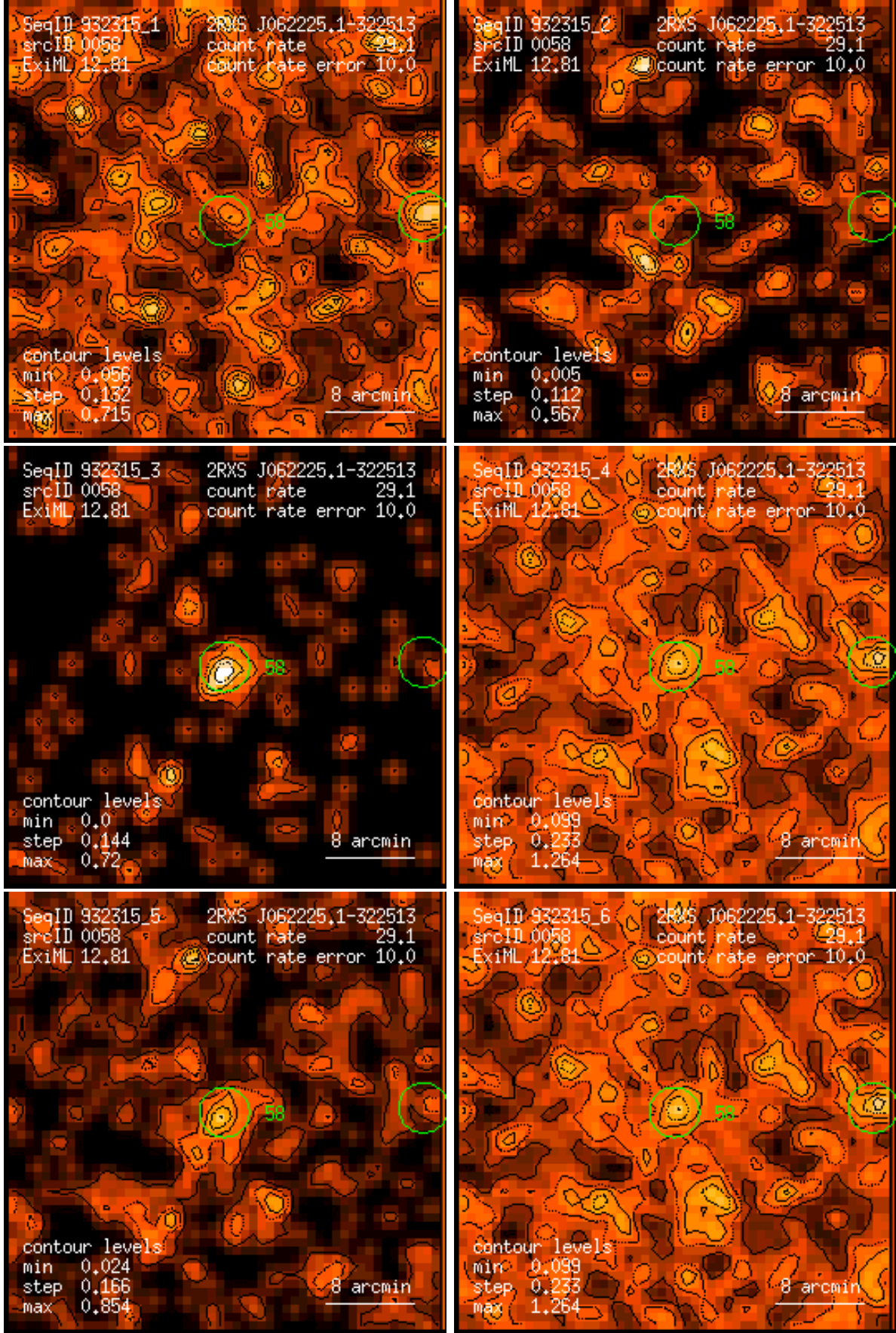
Figure 58: RASS 932315: detection 0058: band rate images, Gaussian filter: (1) PSPC channels 11 – 41, (2) 52 – 90, (3) 91 – 201, (4) 11 – 235, (5) 52 – 201, (6) 11 – 201. Broad band rates in counts/ks. Band rate contour levels in counts/ks/arcmin 2 .
