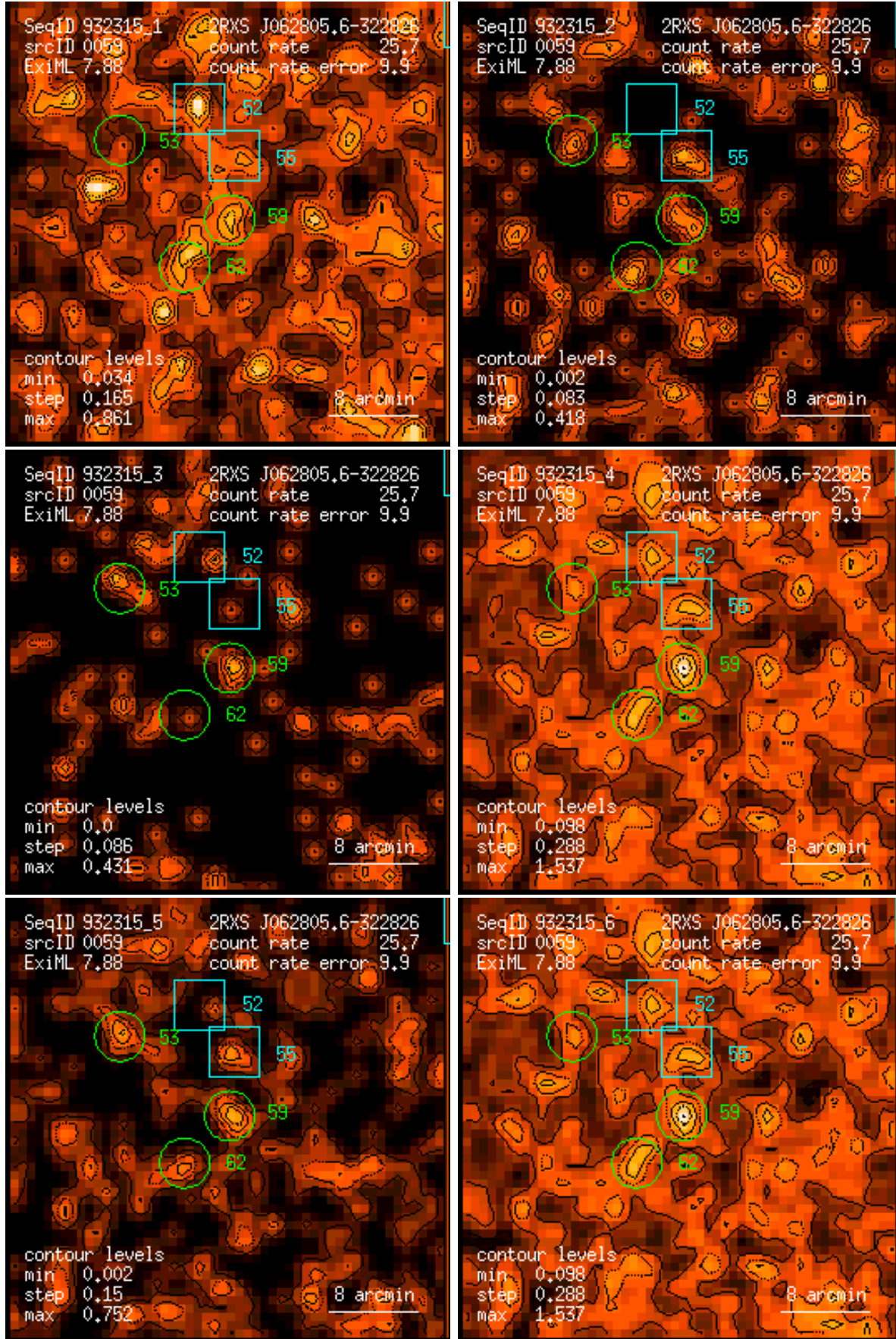
Figure 59: RASS 932315: detection 0059: band rate images, Gaussian filter: (1) PSPC channels 11 – 41, (2) 52 – 90, (3) 91 – 201, (4) 11 – 235, (5) 52 – 201, (6) 11 – 201. Broad band rates in counts/ks. Band rate contour levels in counts/ks/arcmin 2 .
