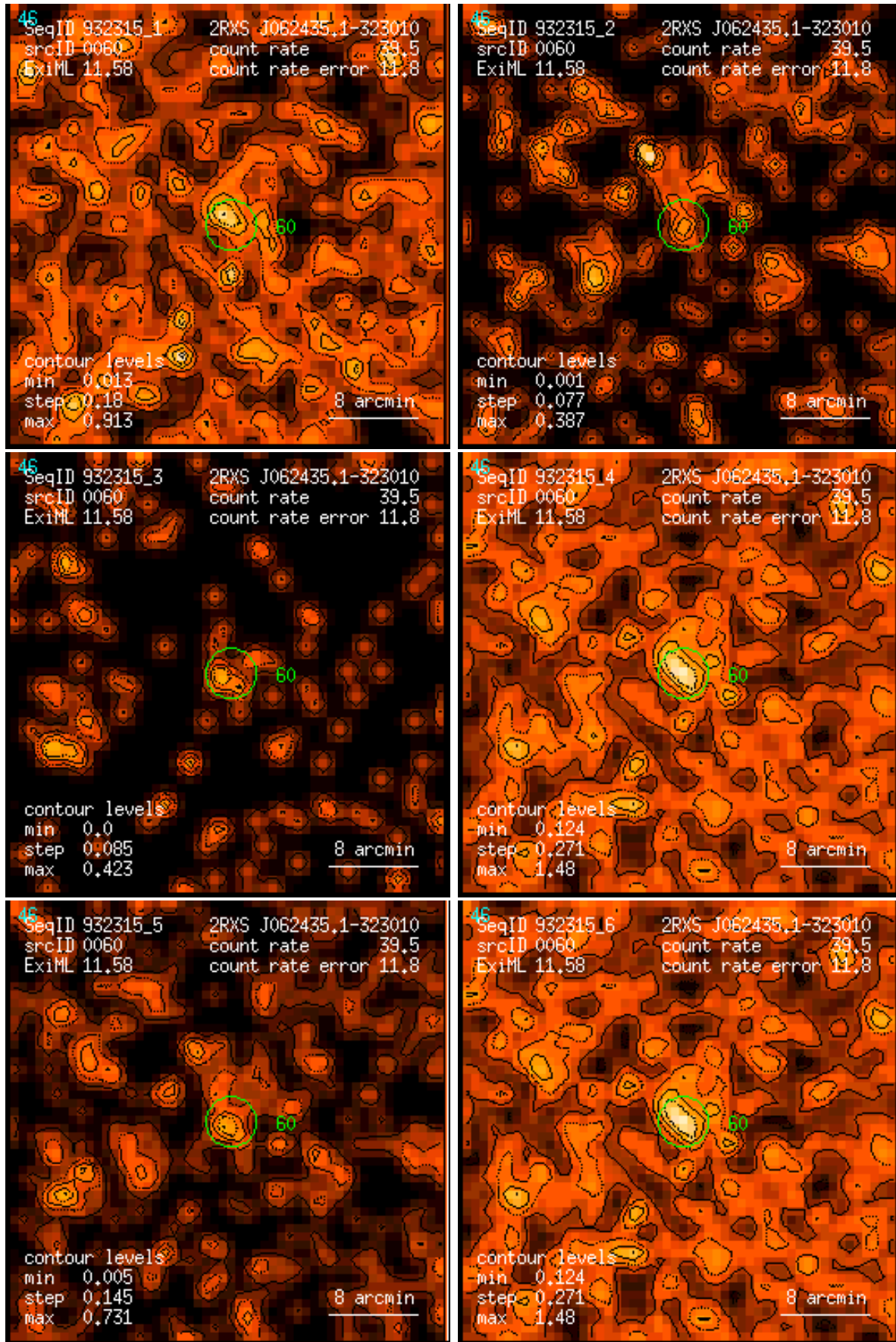
Figure 60: RASS 932315: detection 0060: band rate images, Gaussian filter: (1) PSPC channels 11 – 41, (2) 52 – 90, (3) 91 – 201, (4) 11 – 235, (5) 52 – 201, (6) 11 – 201. Broad band rates in counts/ks. Band rate contour levels in counts/ks/arcmin 2 .
