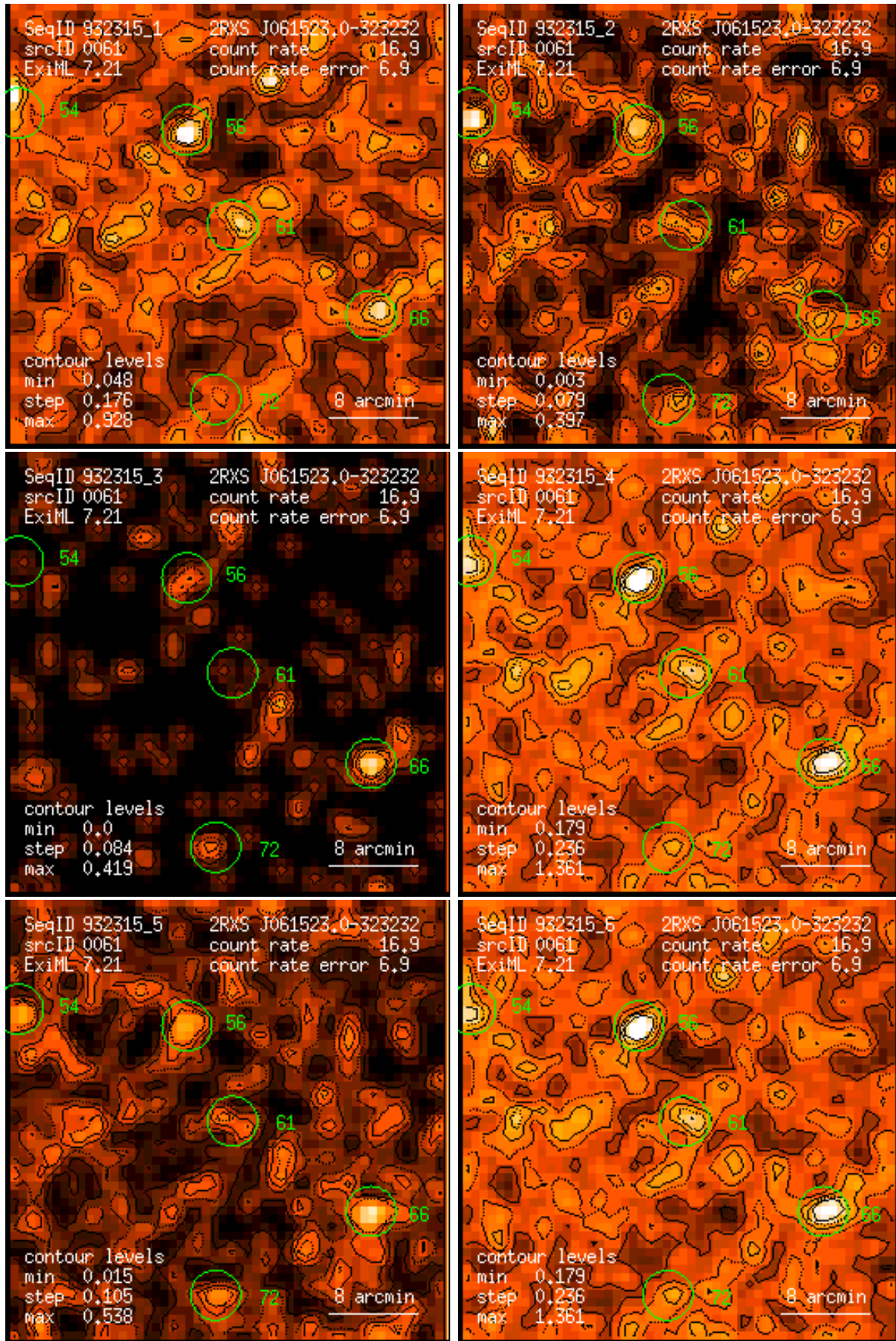
Figure 61: RASS 932315: detection 0061: band rate images, Gaussian filter: (1) PSPC channels 11 – 41, (2) 52 – 90, (3) 91 – 201, (4) 11 – 235, (5) 52 – 201, (6) 11 – 201. Broad band rates in counts/ks. Band rate contour levels in counts/ks/arcmin 2 .
