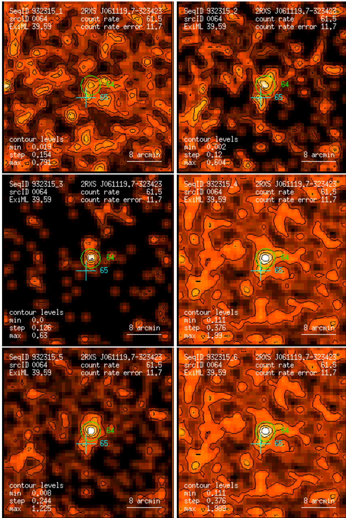
Figure 64: RASS 932315: detection 0064: band rate images, Gaussian filter: (1) PSPC channels 11 – 41, (2) 52 – 90, (3) 91 – 201, (4) 11 – 235, (5) 52 – 201, (6) 11 – 201. Broad band rates in counts/ks. Band rate contour levels in counts/ks/arcmin 2 .
