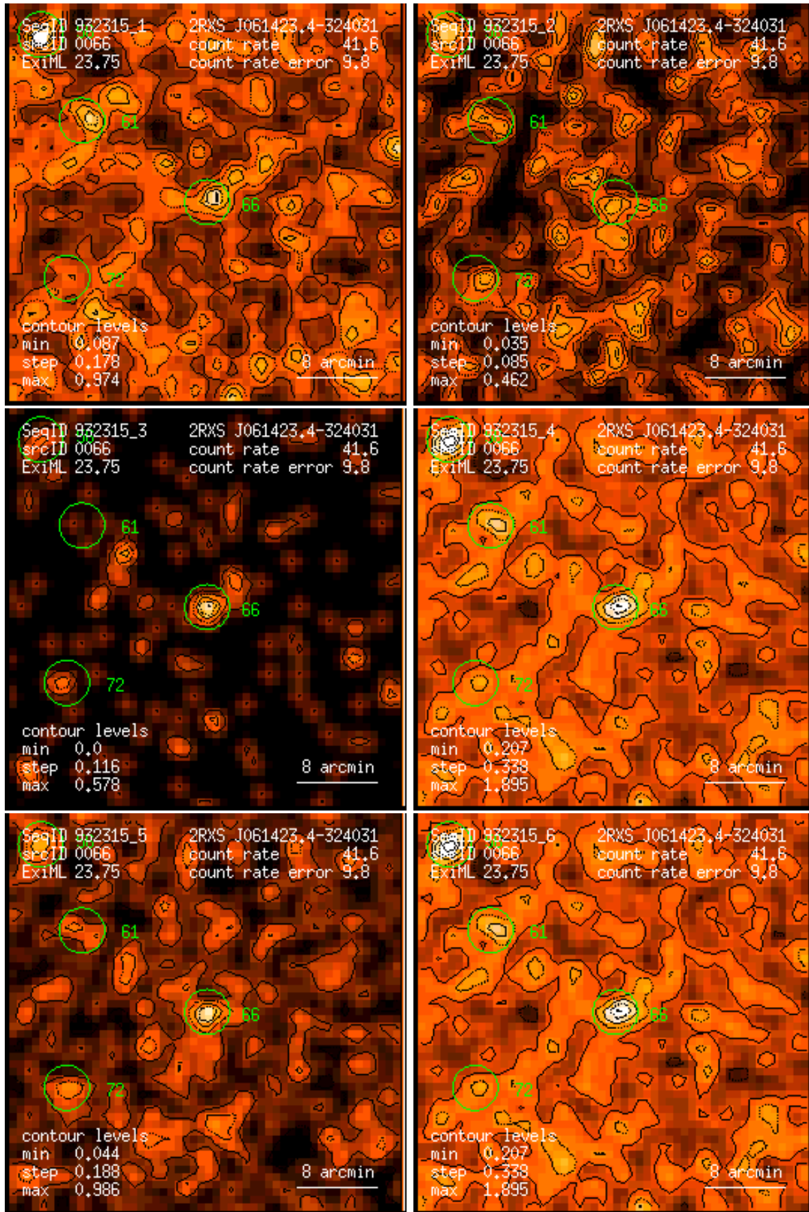
Figure 66: RASS 932315: detection 0066: band rate images, Gaussian filter: (1) PSPC channels 11 – 41, (2) 52 – 90, (3) 91 – 201, (4) 11 – 235, (5) 52 – 201, (6) 11 – 201. Broad band rates in counts/ks. Band rate contour levels in counts/ks/arcmin 2 .
