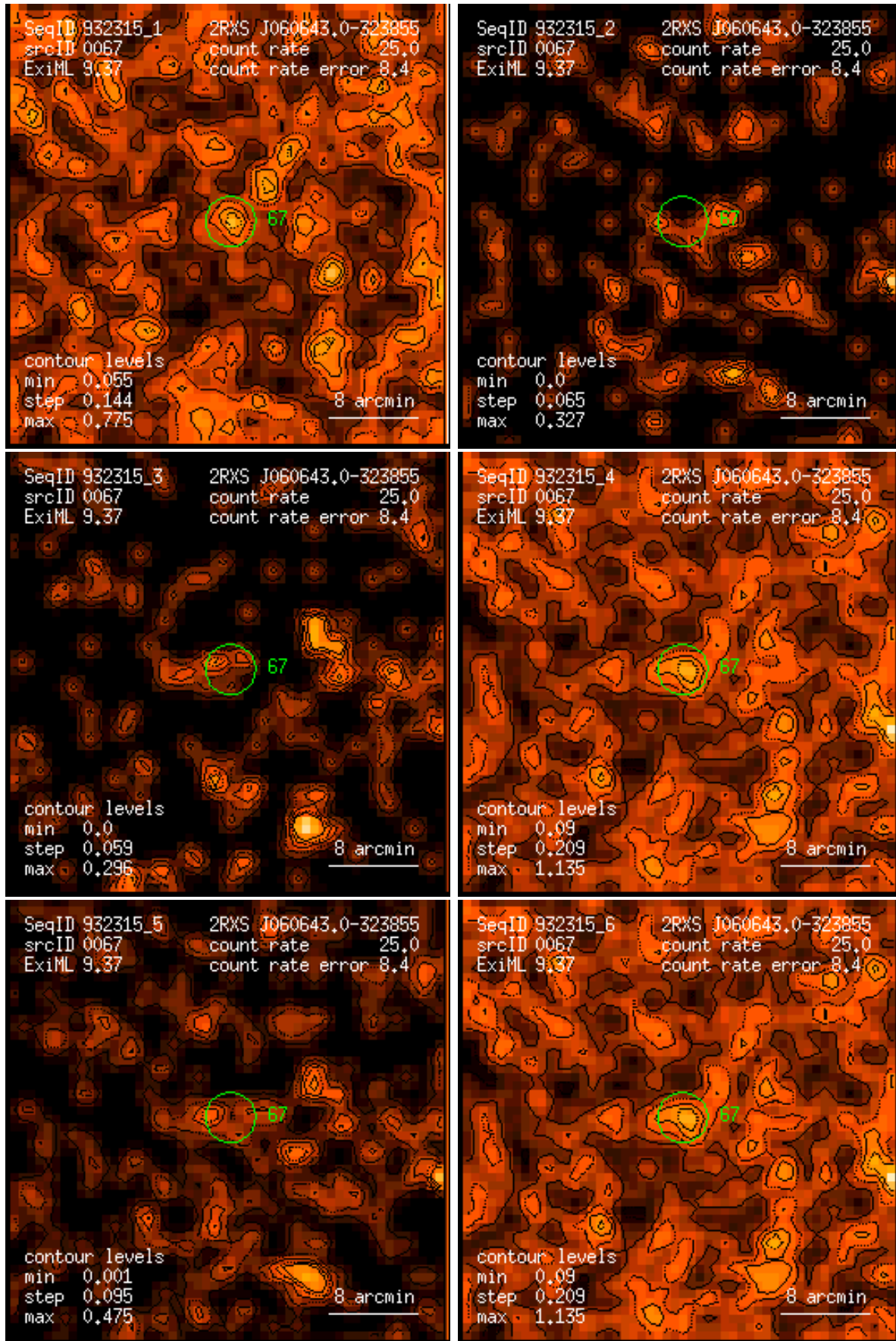
Figure 67: RASS 932315: detection 0067: band rate images, Gaussian filter: (1) PSPC channels 11 – 41, (2) 52 – 90, (3) 91 – 201, (4) 11 – 235, (5) 52 – 201, (6) 11 – 201. Broad band rates in counts/ks. Band rate contour levels in counts/ks/arcmin 2 .
