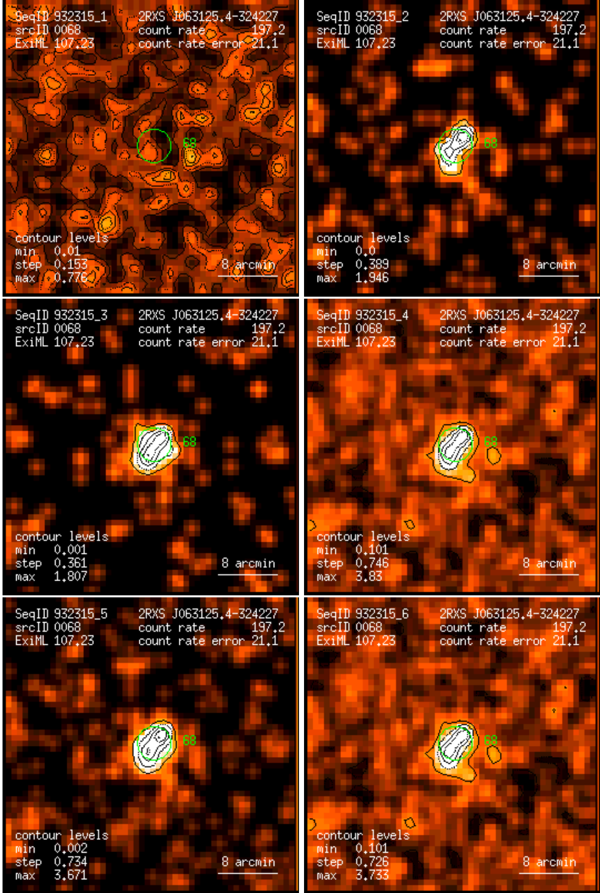
Figure 68: RASS 932315: detection 0068: band rate images, Gaussian filter: (1) PSPC channels 11 – 41, (2) 52 – 90, (3) 91 – 201, (4) 11 – 235, (5) 52 – 201, (6) 11 – 201. Broad band rates in counts/ks. Band rate contour levels in counts/ks/arcmin 2 .
