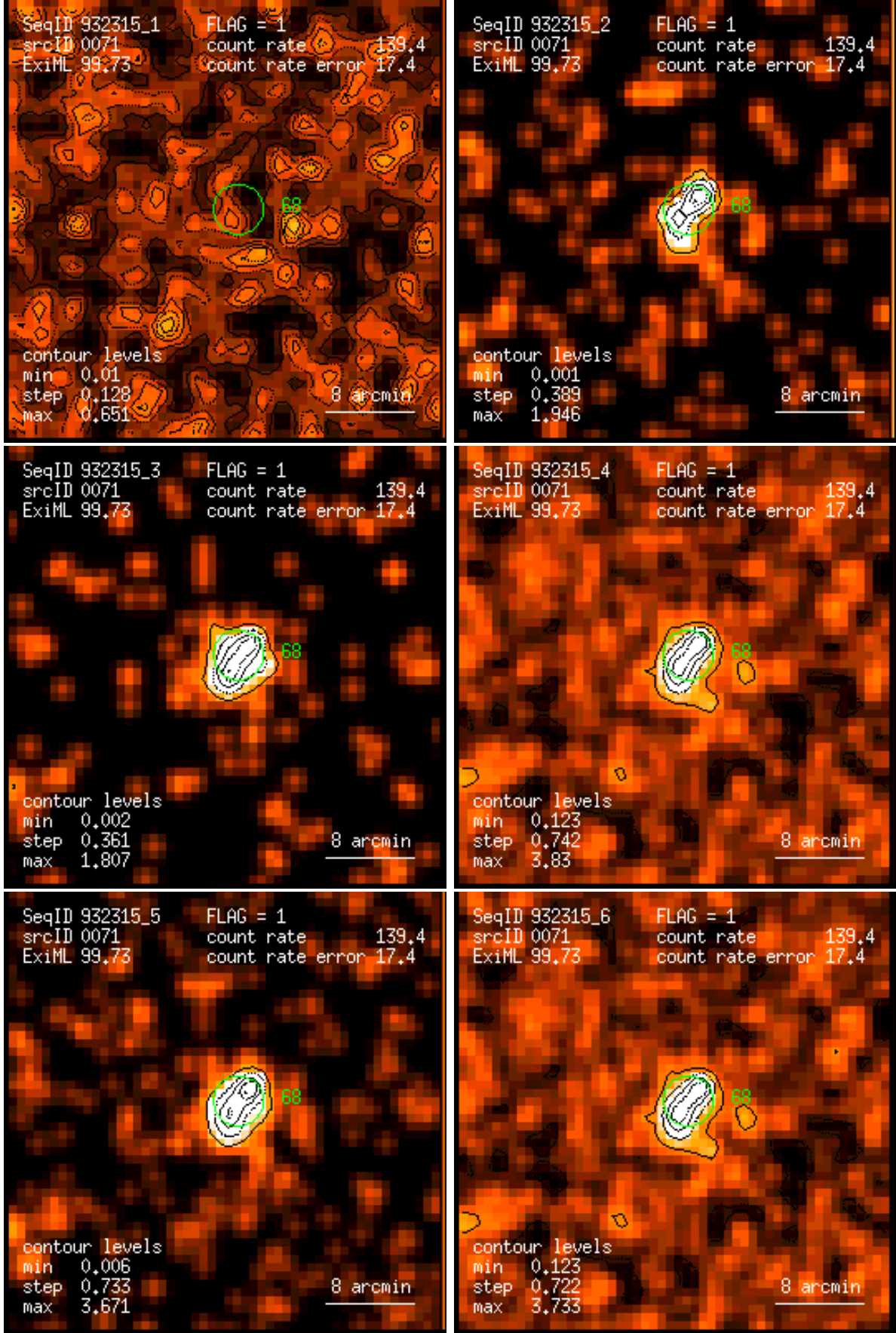
Figure 71: RASS 932315: detection 0071: band rate images, Gaussian filter: (1) PSPC channels 11 – 41, (2) 52 – 90, (3) 91 – 201, (4) 11 – 235, (5) 52 – 201, (6) 11 – 201. Broad band rates in counts/ks. Band rate contour levels in counts/ks/arcmin 2 .
