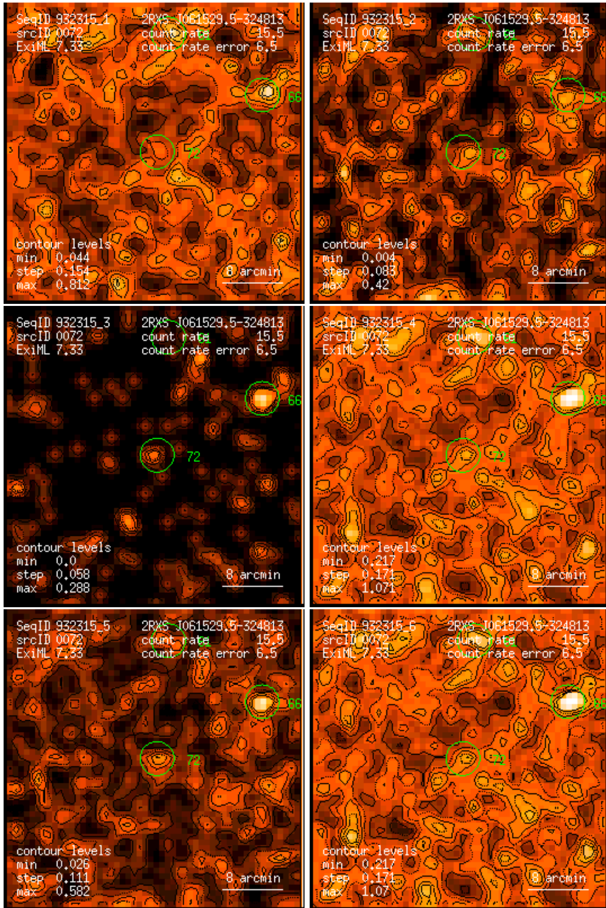
Figure 72: RASS 932315: detection 0072: band rate images, Gaussian filter: (1) PSPC channels 11 – 41, (2) 52 – 90, (3) 91 – 201, (4) 11 – 235, (5) 52 – 201, (6) 11 – 201. Broad band rates in counts/ks. Band rate contour levels in counts/ks/arcmin 2 .
