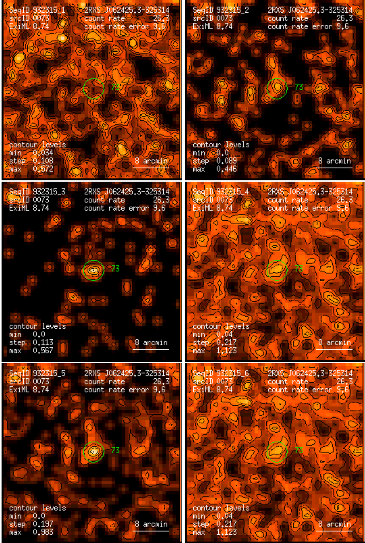
Figure 73: RASS 932315: detection 0073: band rate images, Gaussian filter: (1) PSPC channels 11 – 41, (2) 52 – 90, (3) 91 – 201, (4) 11 – 235, (5) 52 – 201, (6) 11 – 201. Broad band rates in counts/ks. Band rate contour levels in counts/ks/arcmin 2 .
