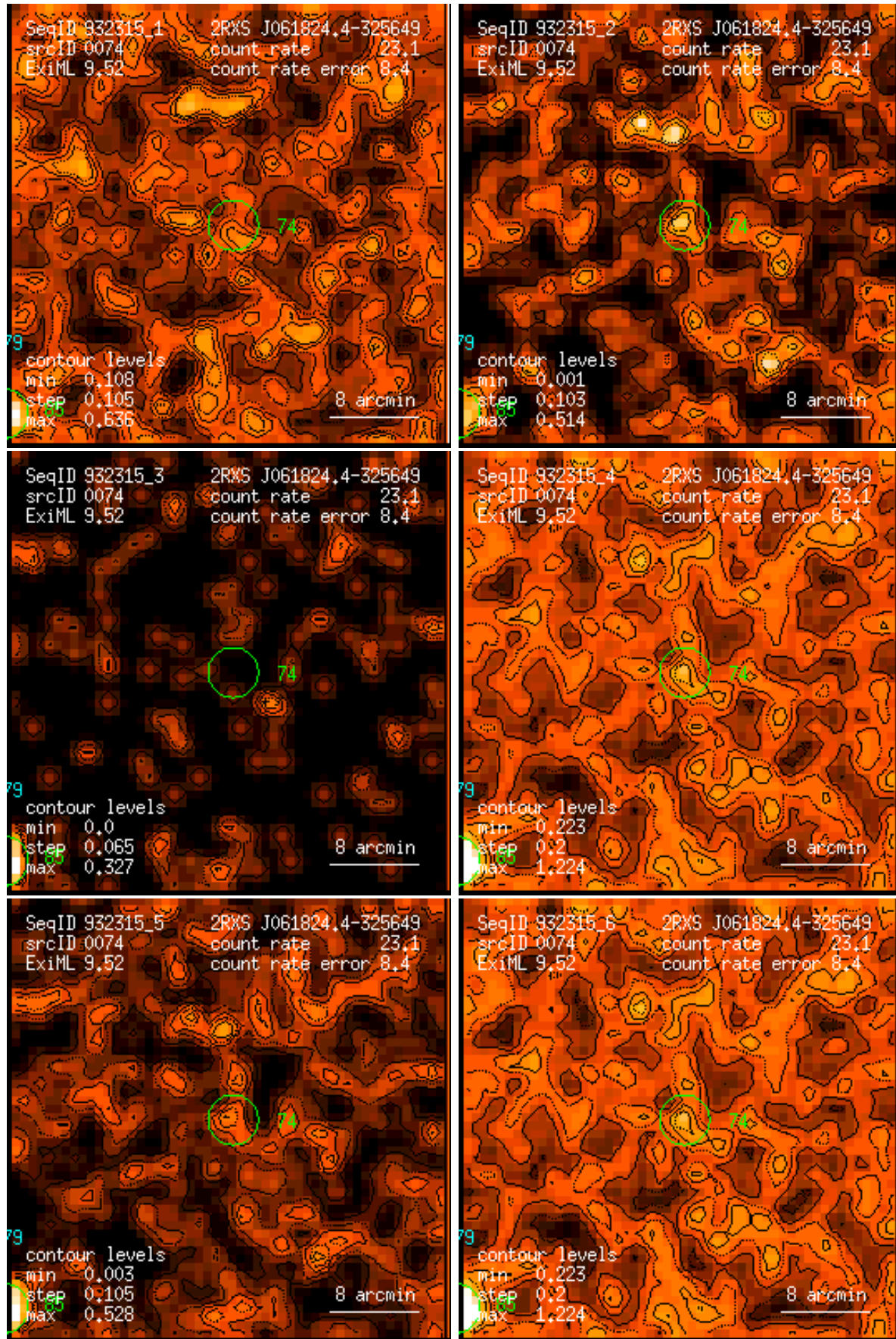
Figure 74: RASS 932315: detection 0074: band rate images, Gaussian filter: (1) PSPC channels 11 – 41, (2) 52 – 90, (3) 91 – 201, (4) 11 – 235, (5) 52 – 201, (6) 11 – 201. Broad band rates in counts/ks. Band rate contour levels in counts/ks/arcmin 2 .
