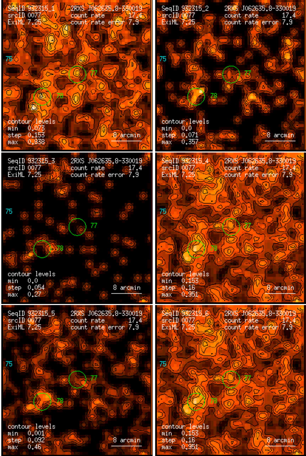
Figure 77: RASS 932315: detection 0077: band rate images, Gaussian filter: (1) PSPC channels 11 – 41, (2) 52 – 90, (3) 91 – 201, (4) 11 – 235, (5) 52 – 201, (6) 11 – 201. Broad band rates in counts/ks. Band rate contour levels in counts/ks/arcmin 2 .
