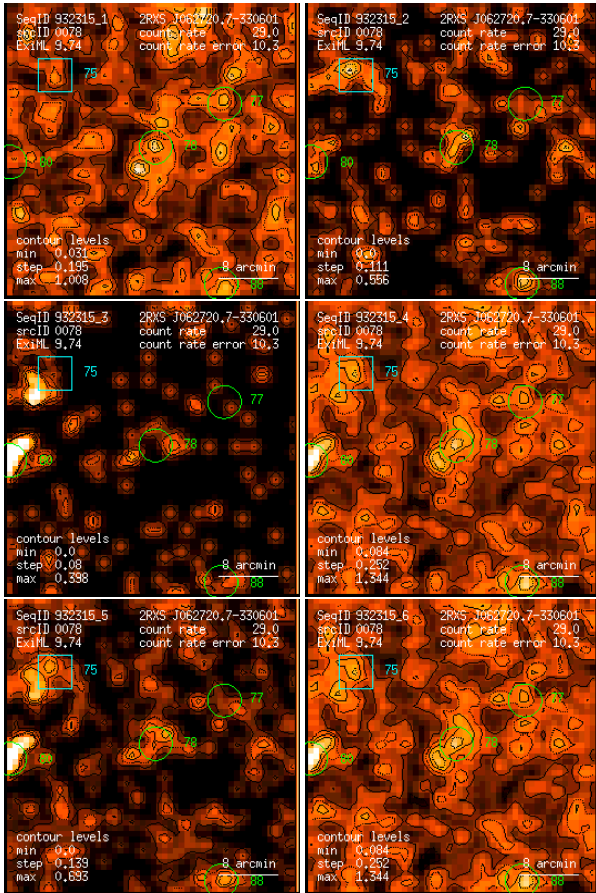
Figure 78: RASS 932315: detection 0078: band rate images, Gaussian filter: (1) PSPC channels 11 – 41, (2) 52 – 90, (3) 91 – 201, (4) 11 – 235, (5) 52 – 201, (6) 11 – 201. Broad band rates in counts/ks. Band rate contour levels in counts/ks/arcmin 2 .
