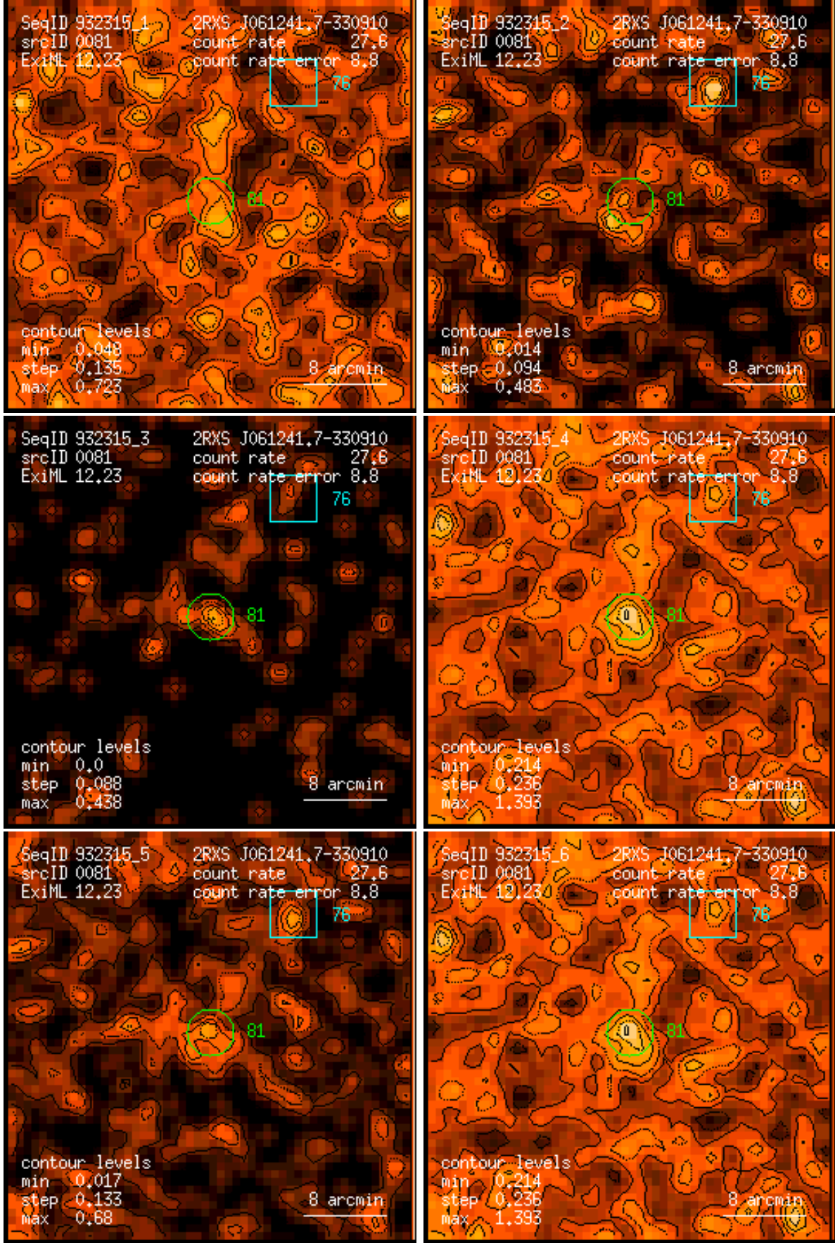
Figure 81: RASS 932315: detection 0081: band rate images, Gaussian filter: (1) PSPC channels 11 – 41, (2) 52 – 90, (3) 91 – 201, (4) 11 – 235, (5) 52 – 201, (6) 11 – 201. Broad band rates in counts/ks. Band rate contour levels in counts/ks/arcmin 2 .
