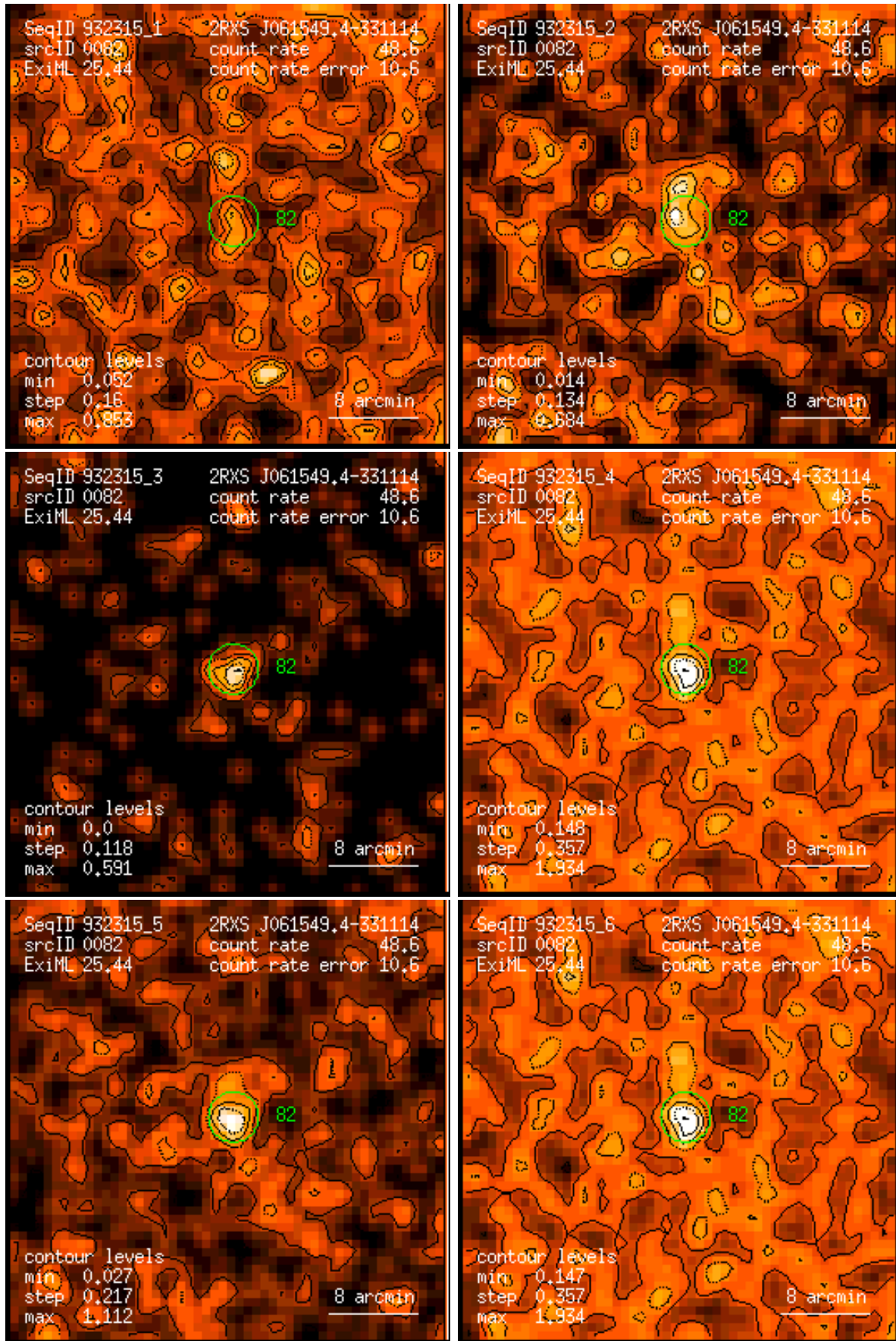
Figure 82: RASS 932315: detection 0082: band rate images, Gaussian filter: (1) PSPC channels 11 – 41, (2) 52 – 90, (3) 91 – 201, (4) 11 – 235, (5) 52 – 201, (6) 11 – 201. Broad band rates in counts/ks. Band rate contour levels in counts/ks/arcmin 2 .
