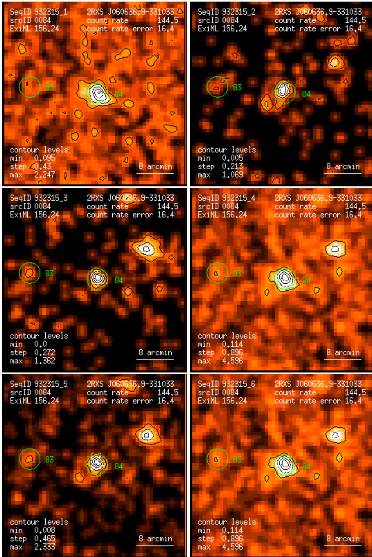
Figure 84: RASS 932315: detection 0084: band rate images, Gaussian filter: (1) PSPC channels 11 – 41, (2) 52 – 90, (3) 91 – 201, (4) 11 – 235, (5) 52 – 201, (6) 11 – 201. Broad band rates in counts/ks. Band rate contour levels in counts/ks/arcmin 2 .
