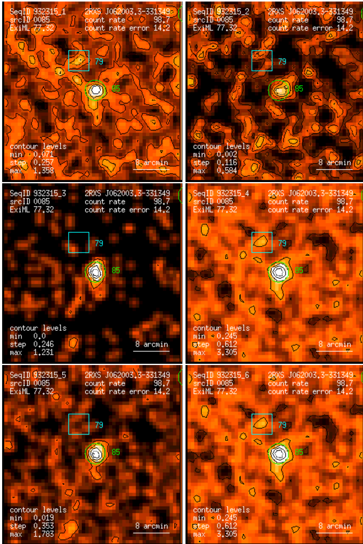
Figure 85: RASS 932315: detection 0085: band rate images, Gaussian filter: (1) PSPC channels 11 – 41, (2) 52 – 90, (3) 91 – 201, (4) 11 – 235, (5) 52 – 201, (6) 11 – 201. Broad band rates in counts/ks. Band rate contour levels in counts/ks/arcmin 2 .
