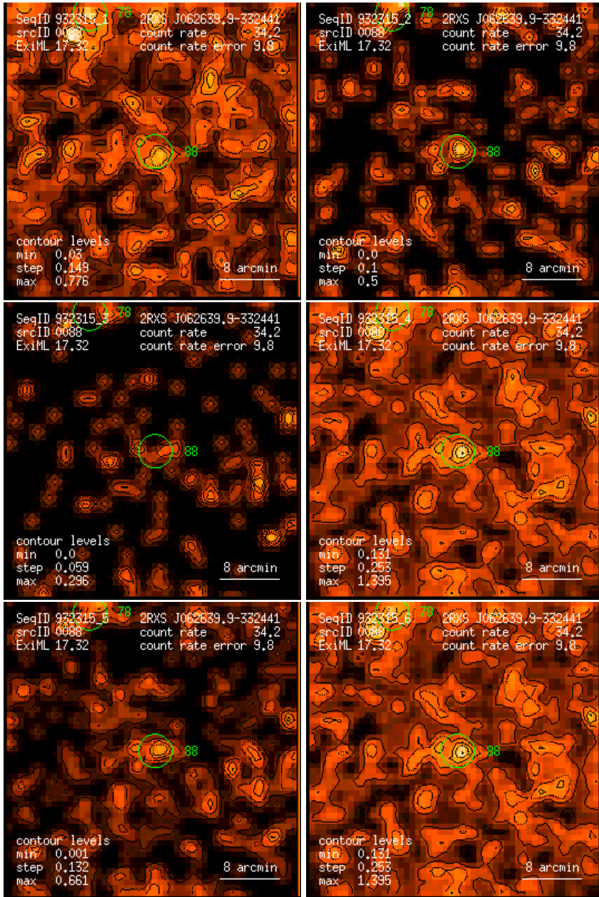
Figure 88: RASS 932315: detection 0088: band rate images, Gaussian filter: (1) PSPC channels 11 – 41, (2) 52 – 90, (3) 91 – 201, (4) 11 – 235, (5) 52 – 201, (6) 11 – 201. Broad band rates in counts/ks. Band rate contour levels in counts/ks/arcmin 2 .
