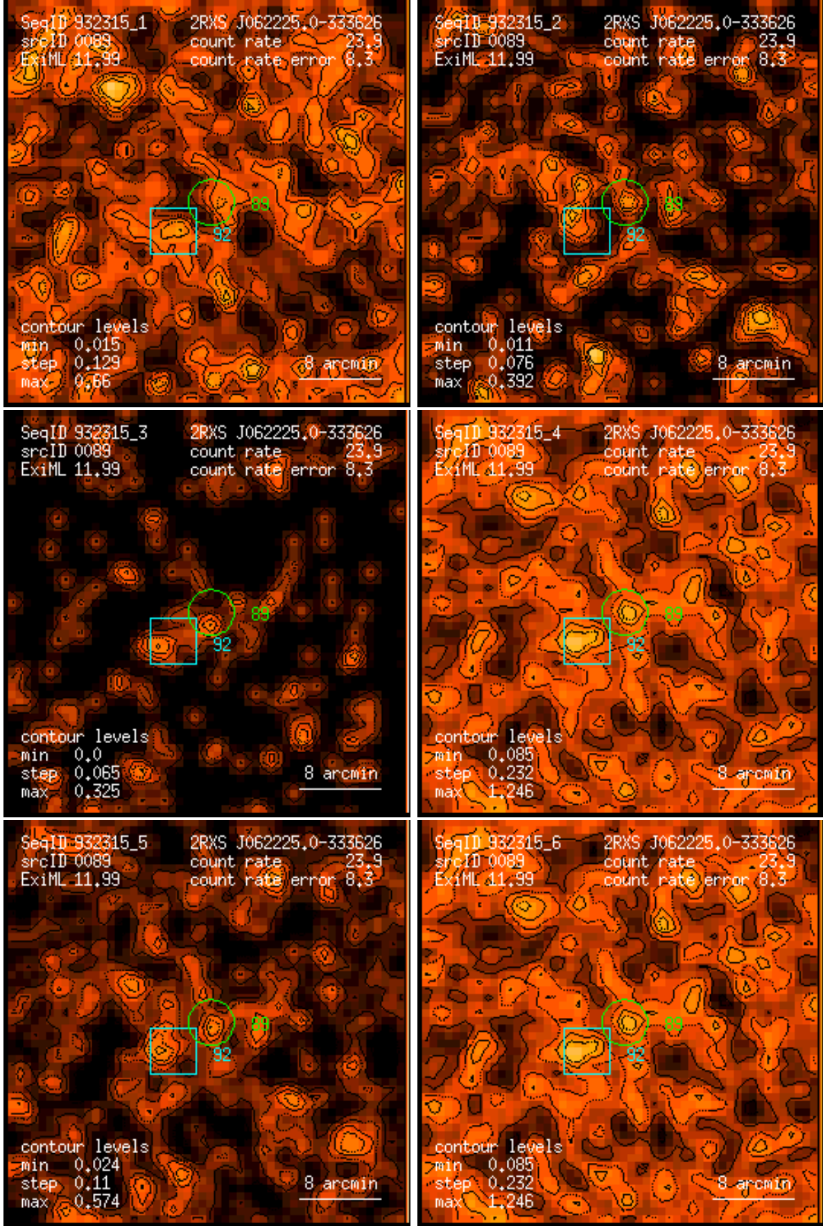
Figure 89: RASS 932315: detection 0089: band rate images, Gaussian filter: (1) PSPC channels 11 – 41, (2) 52 – 90, (3) 91 – 201, (4) 11 – 235, (5) 52 – 201, (6) 11 – 201. Broad band rates in counts/ks. Band rate contour levels in counts/ks/arcmin 2 .
