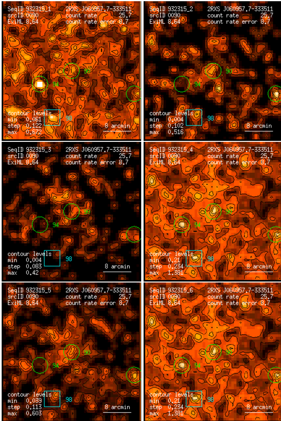
Figure 90: RASS 932315: detection 0090: band rate images, Gaussian filter: (1) PSPC channels 11 – 41, (2) 52 – 90, (3) 91 – 201, (4) 11 – 235, (5) 52 – 201, (6) 11 – 201. Broad band rates in counts/ks. Band rate contour levels in counts/ks/arcmin 2 .
