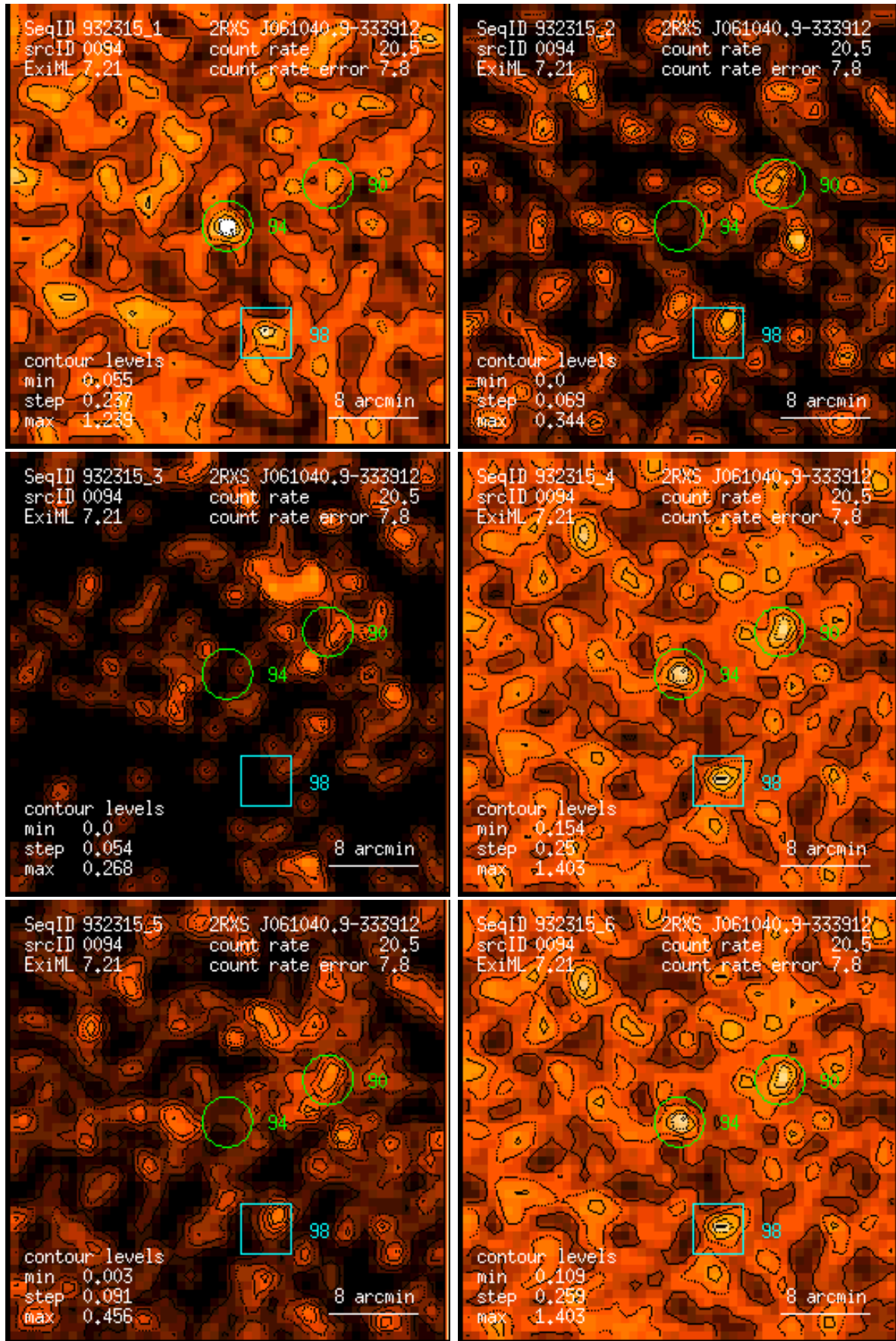
Figure 94: RASS 932315: detection 0094: band rate images, Gaussian filter: (1) PSPC channels 11 – 41, (2) 52 – 90, (3) 91 – 201, (4) 11 – 235, (5) 52 – 201, (6) 11 – 201. Broad band rates in counts/ks. Band rate contour levels in counts/ks/arcmin 2 .
