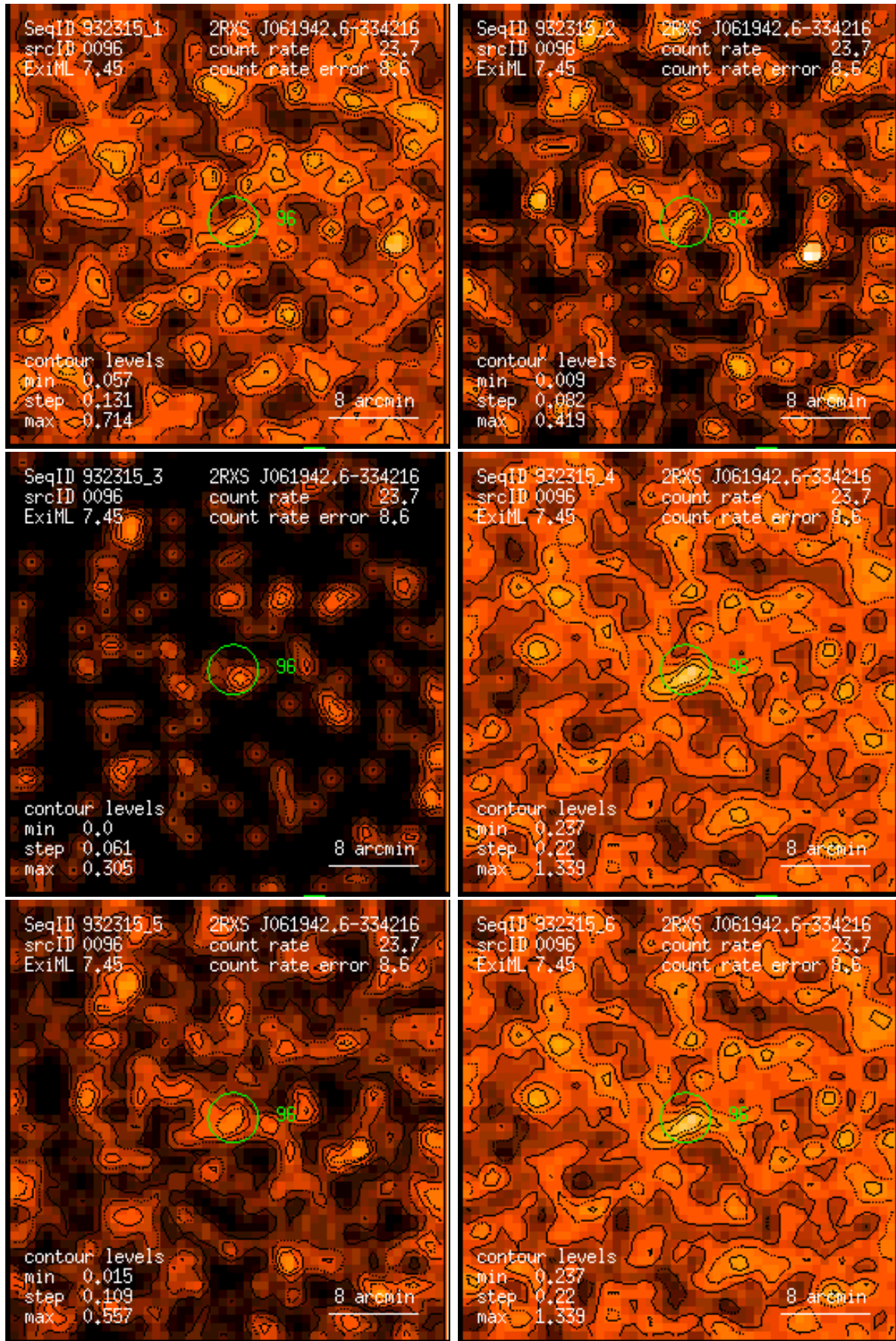
Figure 96: RASS 932315: detection 0096: band rate images, Gaussian filter: (1) PSPC channels 11 – 41, (2) 52 – 90, (3) 91 – 201, (4) 11 – 235, (5) 52 – 201, (6) 11 – 201. Broad band rates in counts/ks. Band rate contour levels in counts/ks/arcmin 2 .
