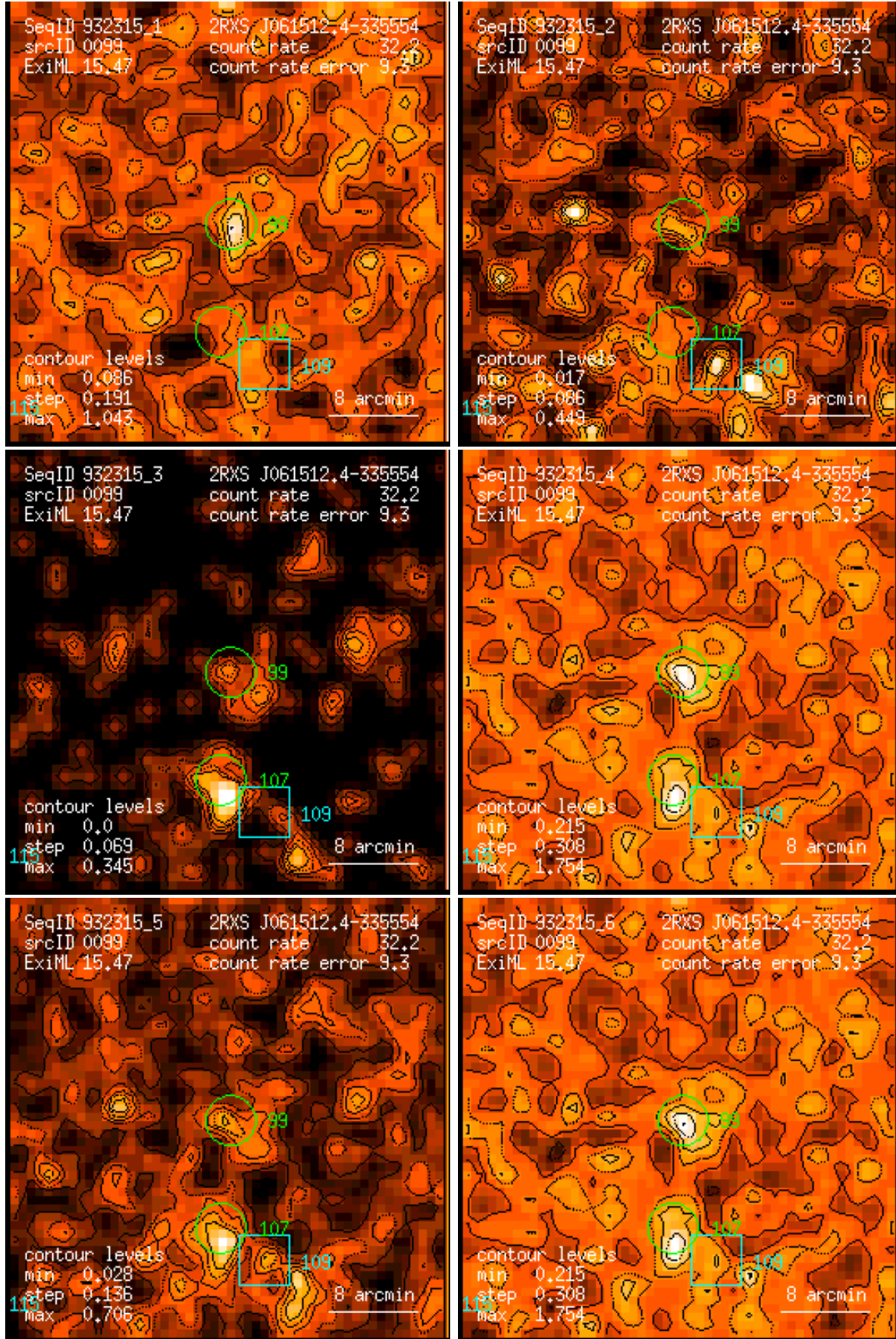
Figure 99: RASS 932315: detection 0099: band rate images, Gaussian filter: (1) PSPC channels 11 – 41, (2) 52 – 90, (3) 91 – 201, (4) 11 – 235, (5) 52 – 201, (6) 11 – 201. Broad band rates in counts/ks. Band rate contour levels in counts/ks/arcmin 2 .
